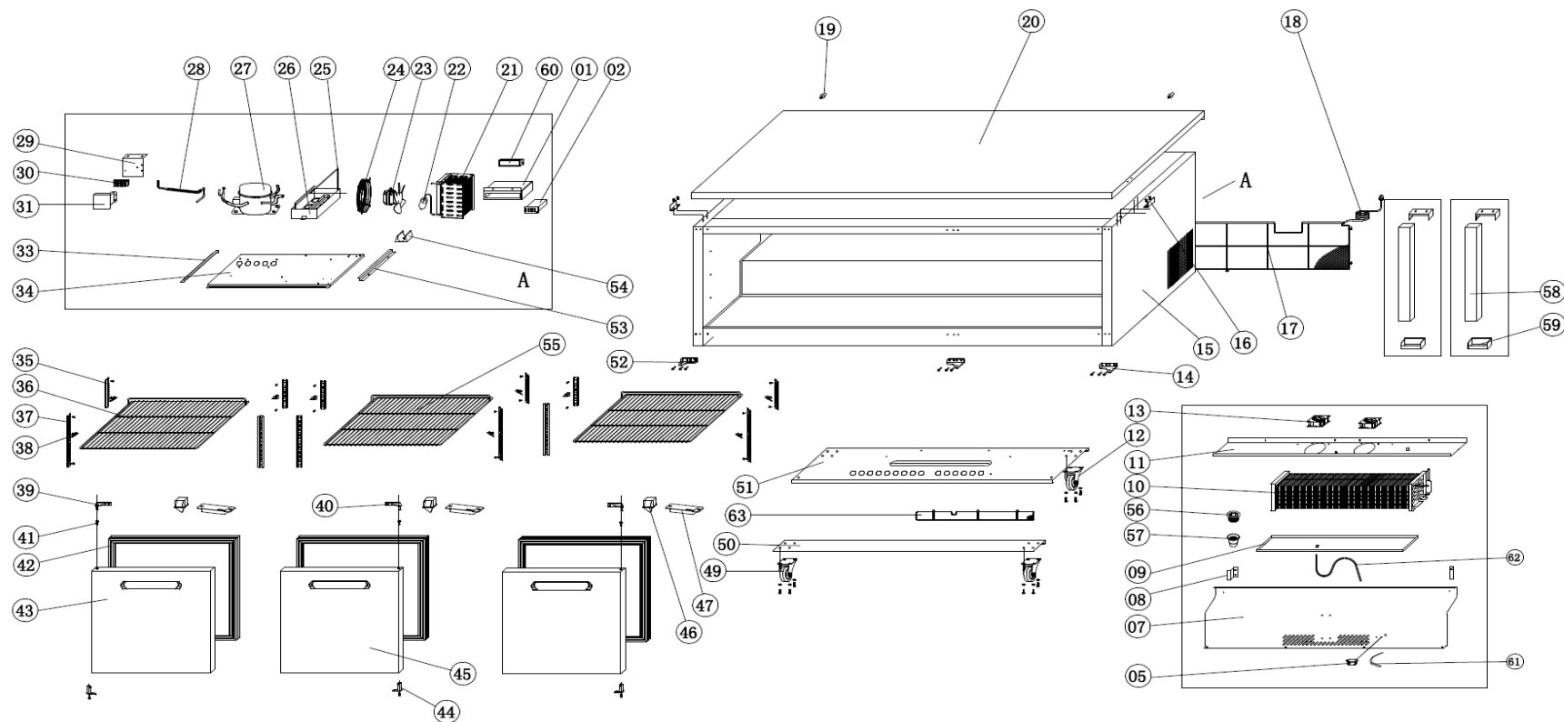
EXPLODE OF KCHUC72R
