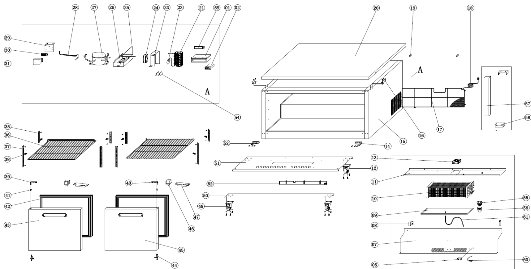
EXPLODE OF KCHUC60R
