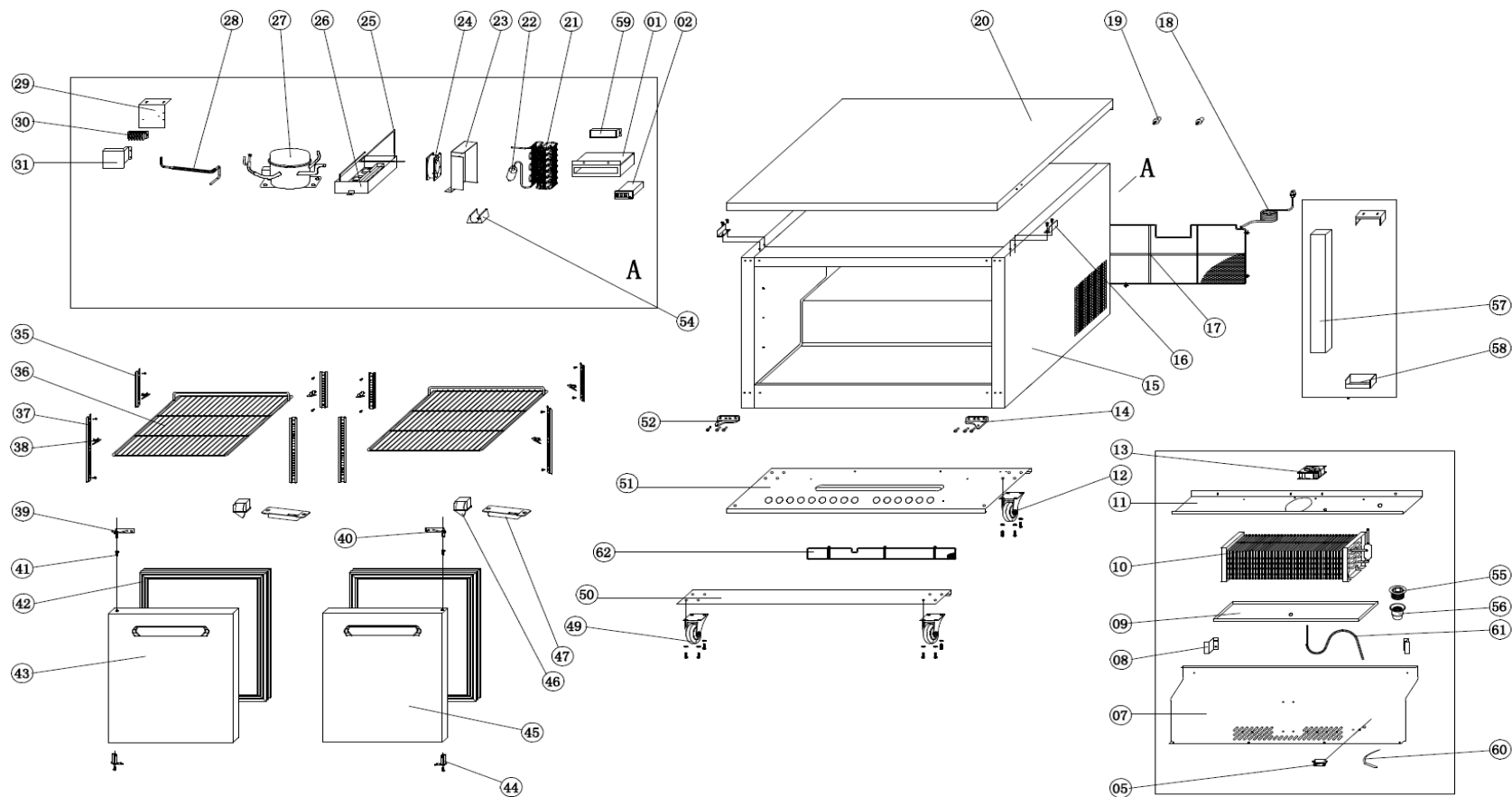
EXPLODE OF KCHUC48R
