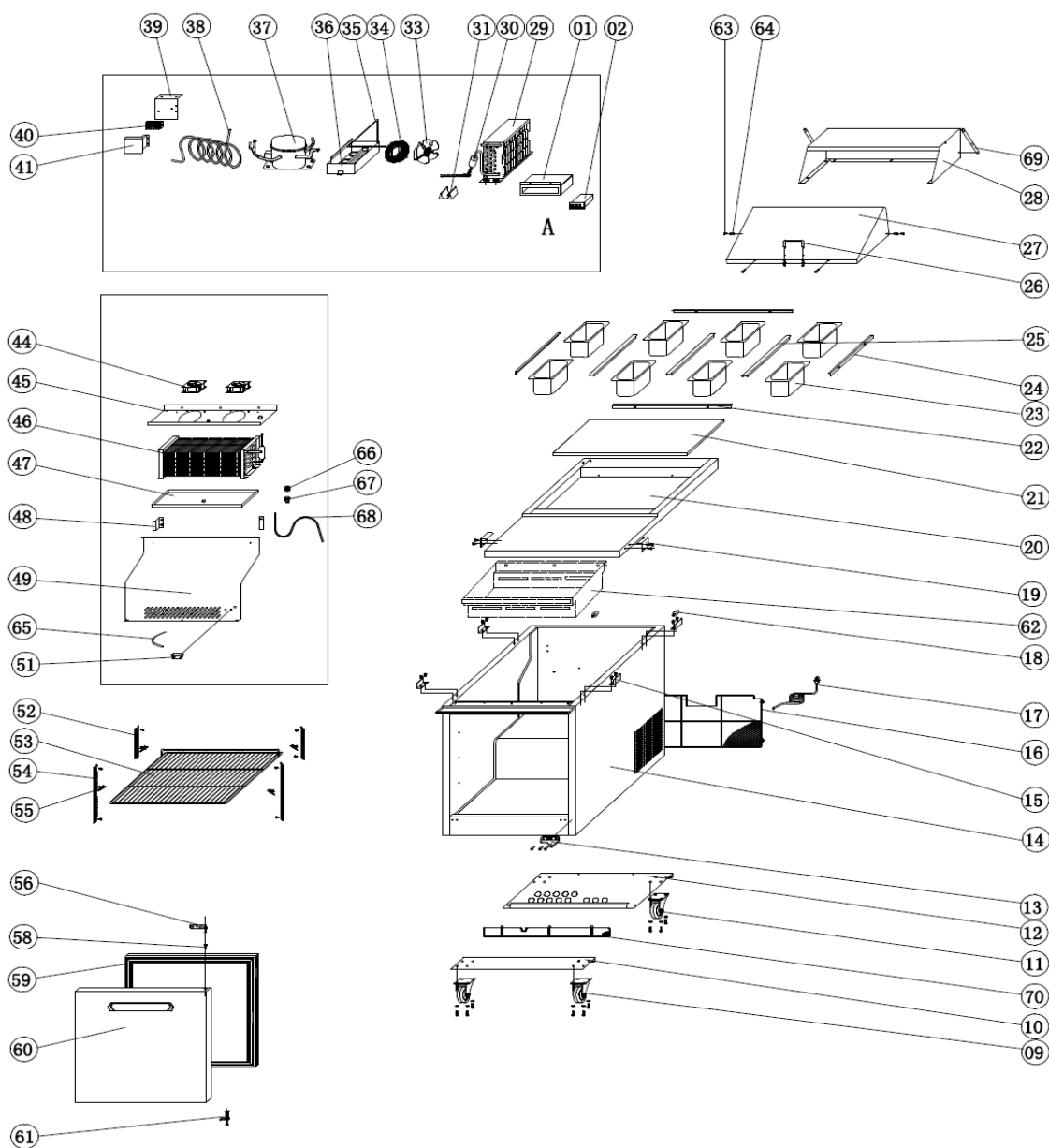
EXPLODE OF KCHST27.8
