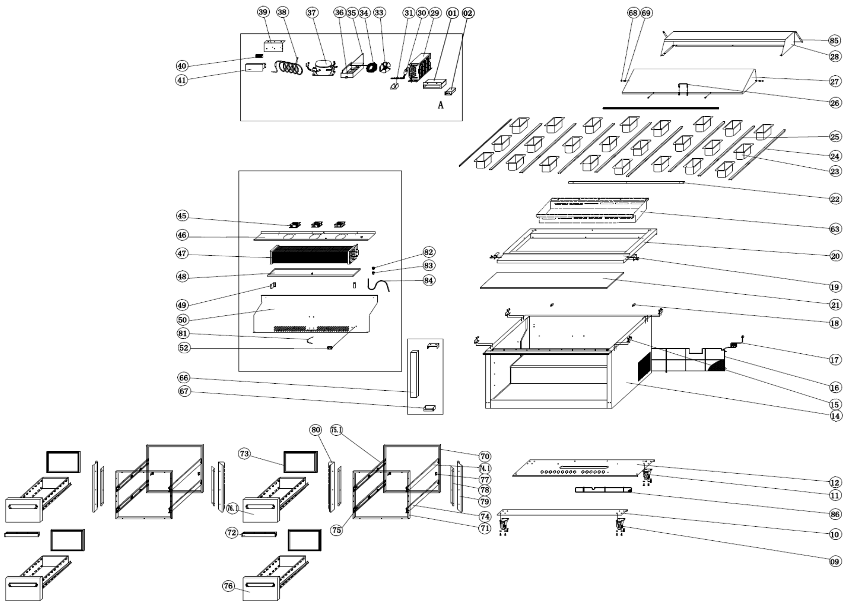
EXPLODE OF KCHMT60.24.4D
