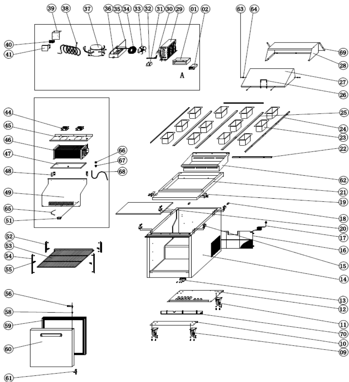
EXPLODE OF KCHMT29.12
