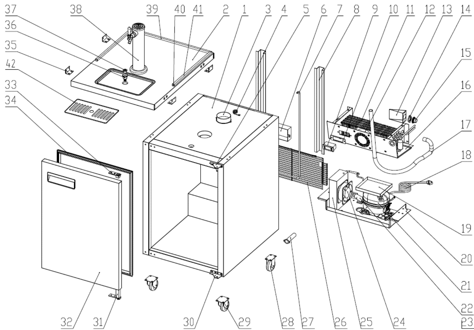
EXPLODED OF KCHBBD1D1T
