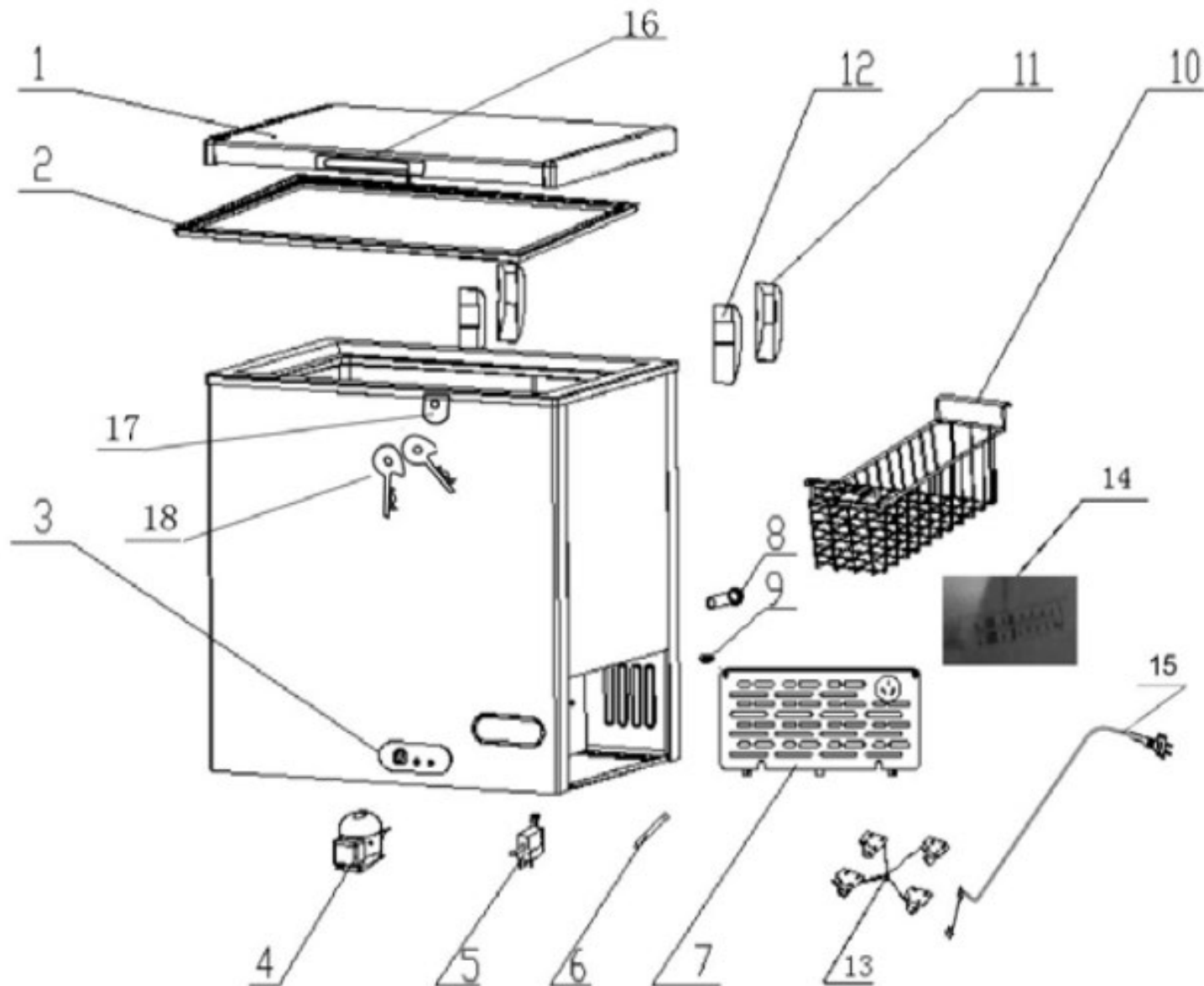
Explosion View Of KCCF073WS
