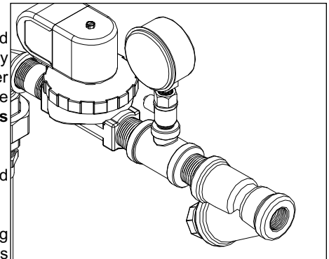
Incoming Plumbing Y-strainer Connection
