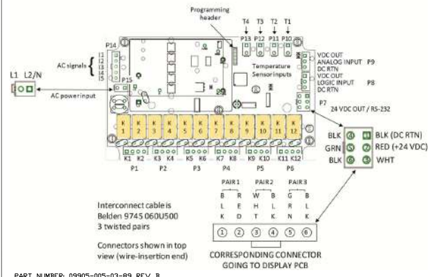
Connection Diagram for I/O Module
