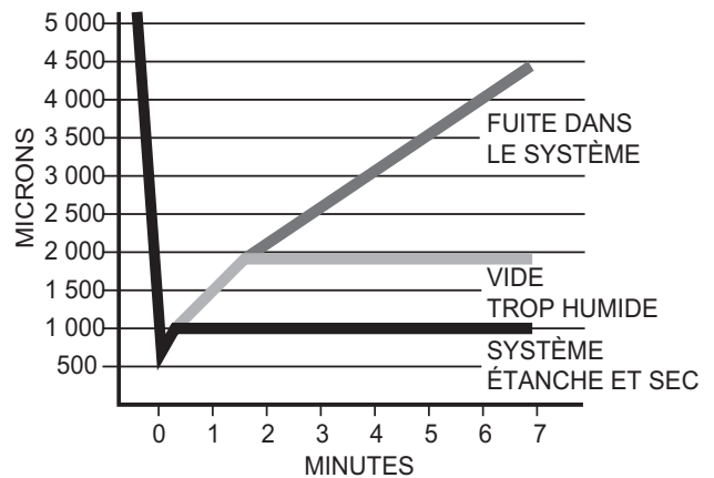
Figure 9 – Courbe de vide
