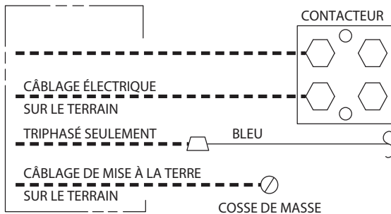
Figure 10 – Raccords de conduite
