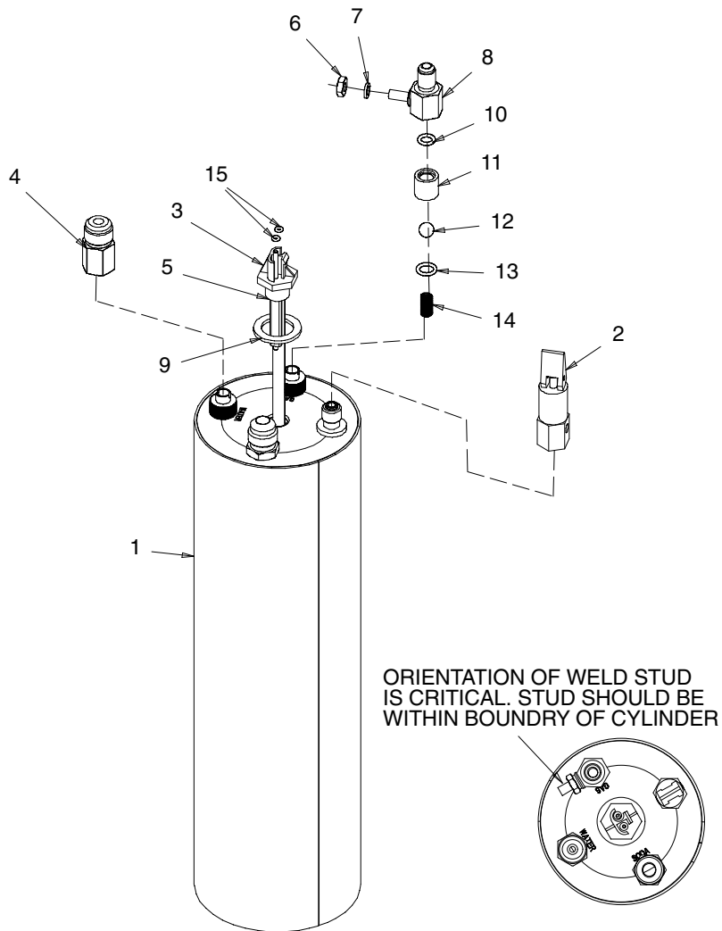
FIGURE 9. CARBONATOR ASSEMBLY
