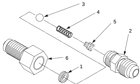
FIGURE 5. CHECK VALVE ASSEMBLY
