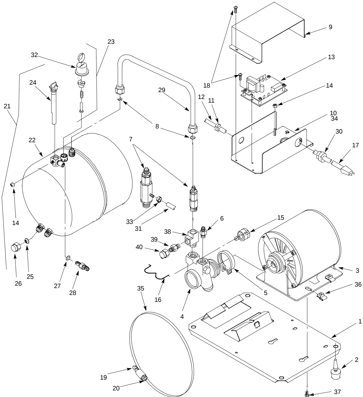
FIGURE 1. LARGE RESERVE CARBONATOR LOW PROFILE ASSEMBLY
