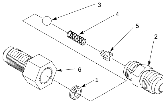
FIGURE 3. CO 2 CHECK VALVE ASSEMBLY
