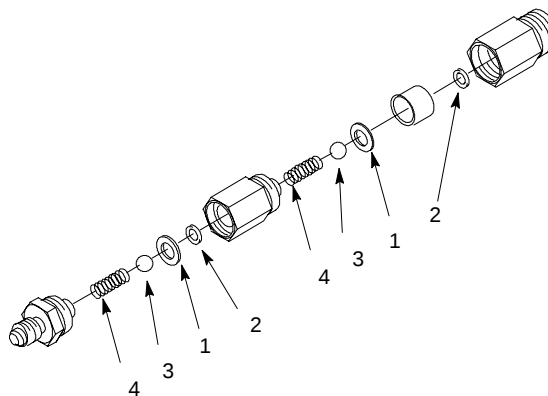
FIGURE 2. LIQUID DUAL CHECK VALVE ASSEMBLY
