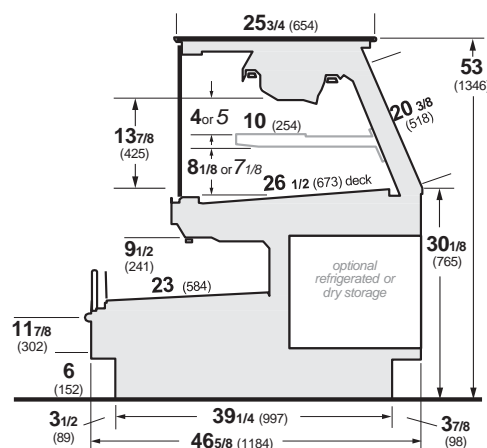
VR3HV-M/F-EP Vertical Glass Meat High Volume Service Dome, Multi Deck Self Service
