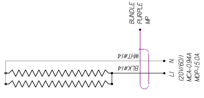
ANTI-SWEAT HEATER 120 VAC III 0495007 40W, 33A III 0497590 50W, 42A
