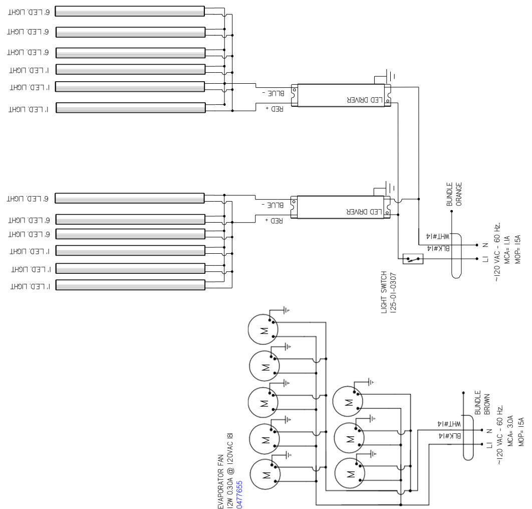
LIGHT CIRCUIT 084A 91.2W @ 120V
