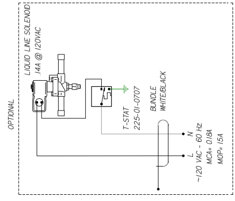
CIRCUIT #2
