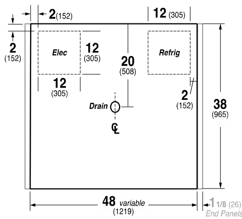
SGB Plan View
