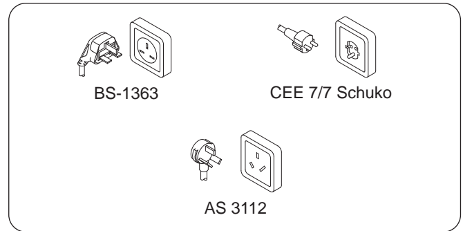
Plug Configurations
