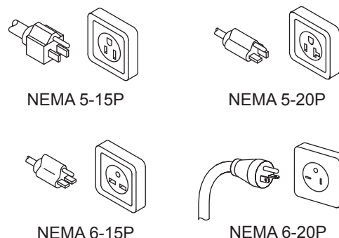
Plug Configurations
