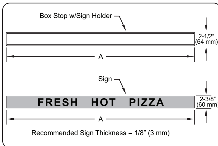
Box Stop with Sign Holder Dimensions
