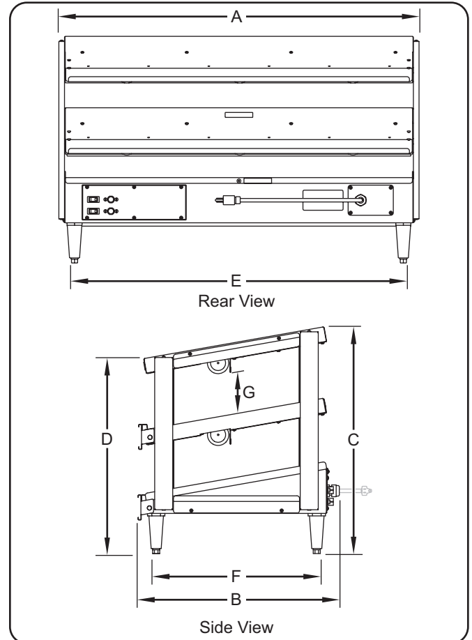
GRPWS-xxxxD Dimensions
