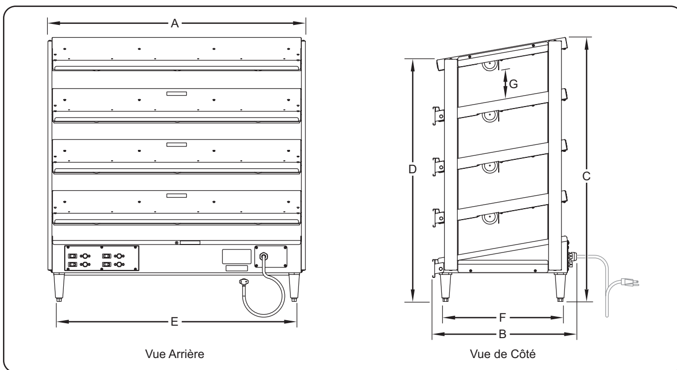
GRPWS-xxxxQ Dimensions
