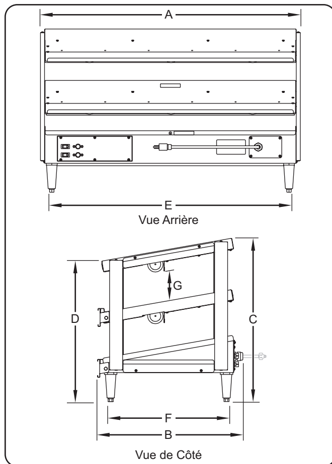
GRPWS-xxxxD Dimensions
