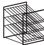
3-Shelf Angle Rack Rack Openings: 4" (102 mm) Middle shelf is removable. Rack shelves slant at 15° angle.
