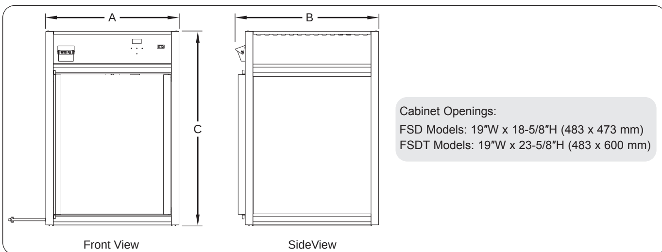
Figure 4. Dimensions
