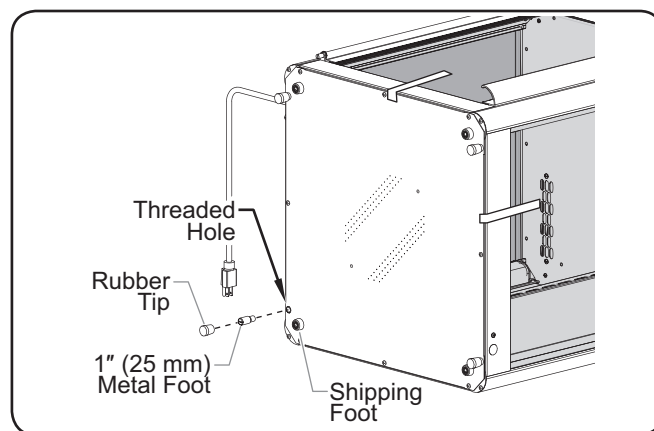
Installing the 1" (25 mm) Feet
