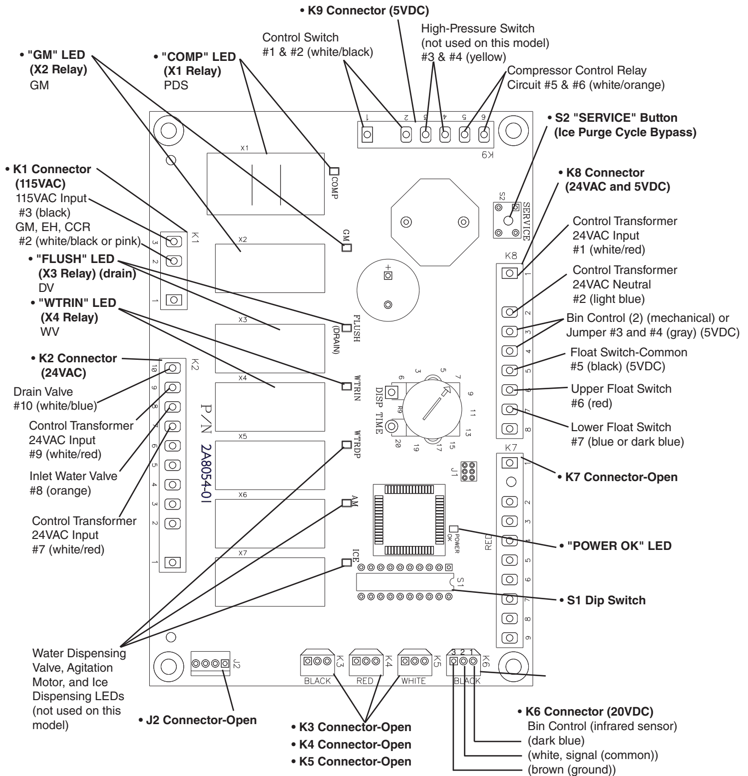
"F-C" Control Board Part Number 2A8054-01
