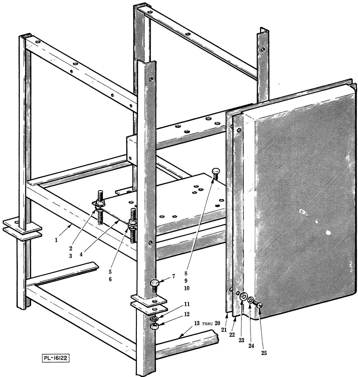
BASE UNIT
