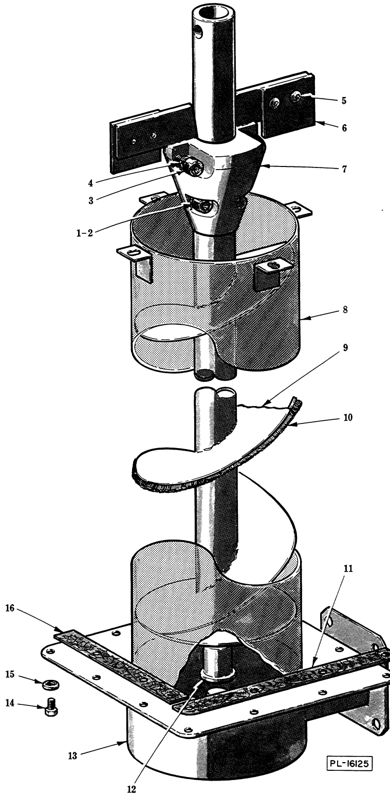
WATER PRESS SCREW UNIT
