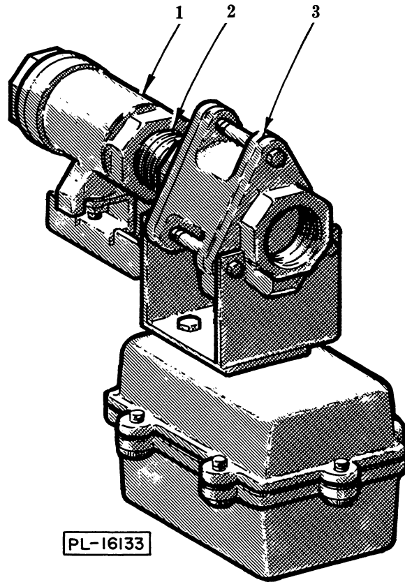
DRAIN VALVE UNIT
