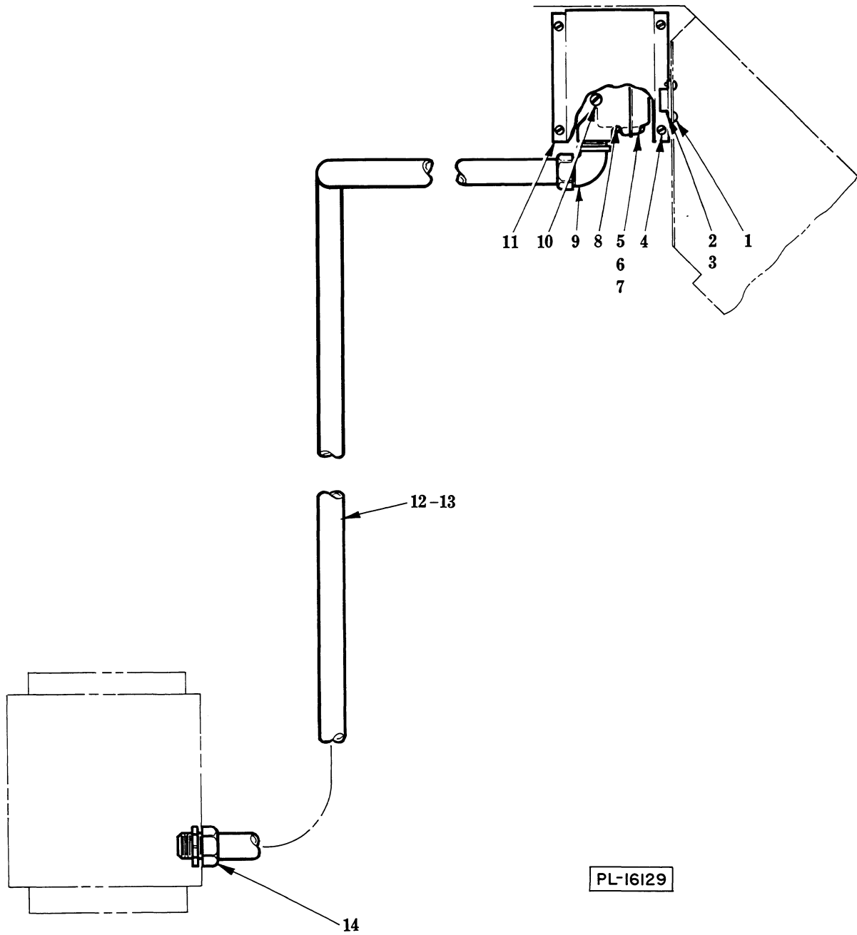
SAFETY SWITCH UNIT (STANDARD CHUTE)
