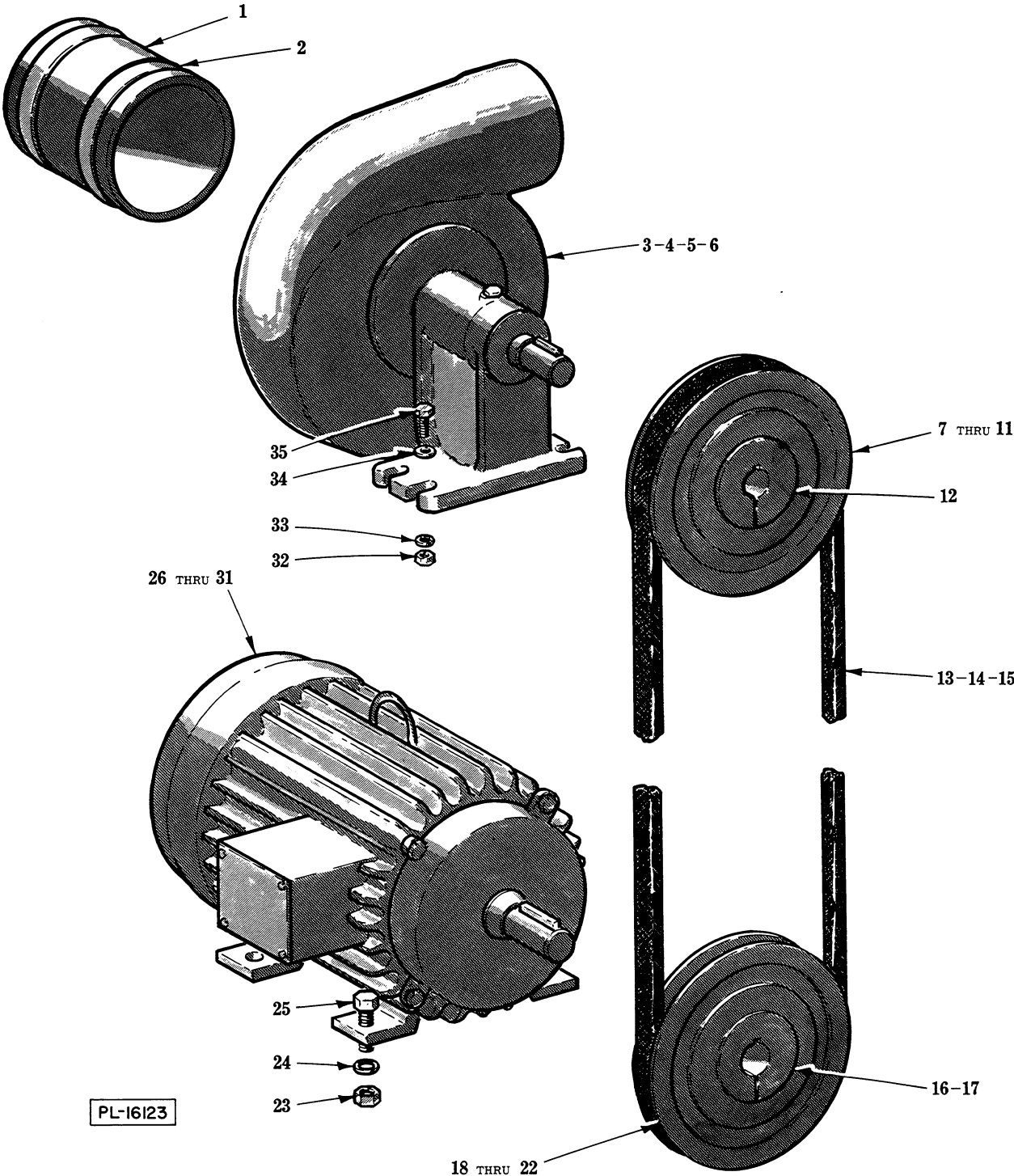
MOTOR AND PUMP UNIT
