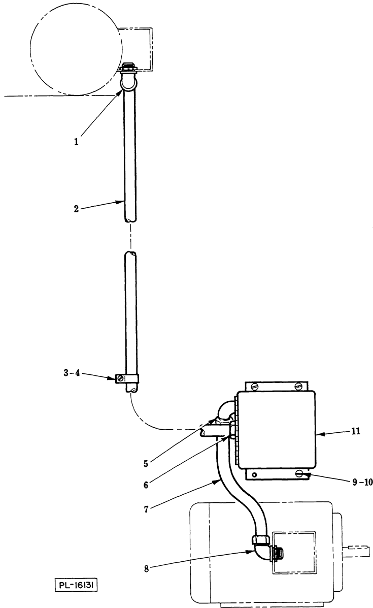
CONDUIT (L. TO R. OPERATION)
