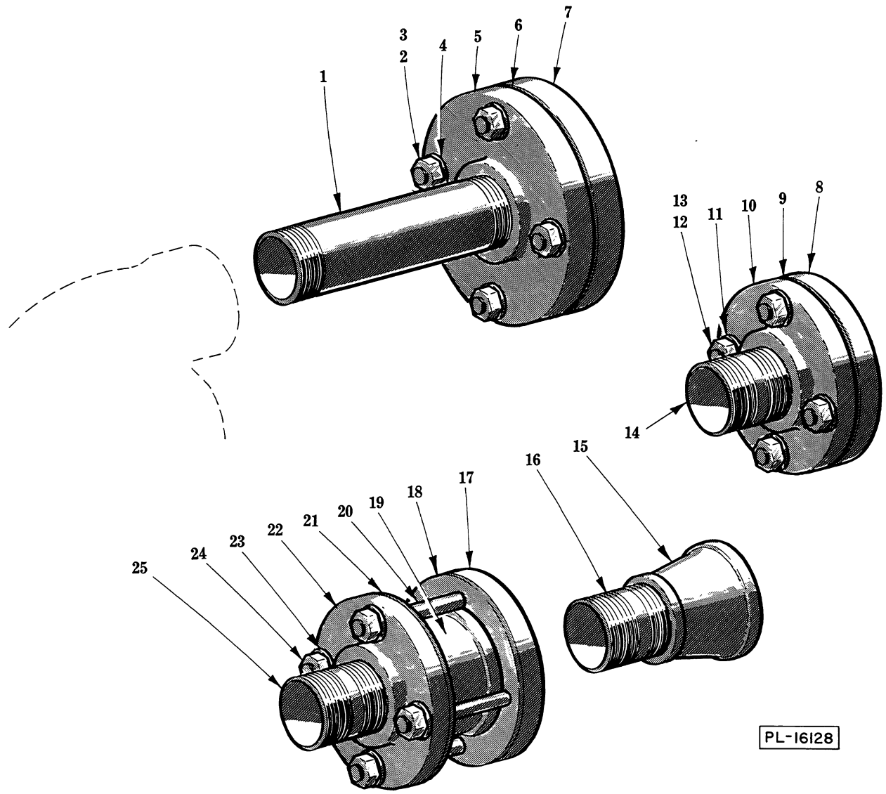
DISCHARGE PIPING UNIT
