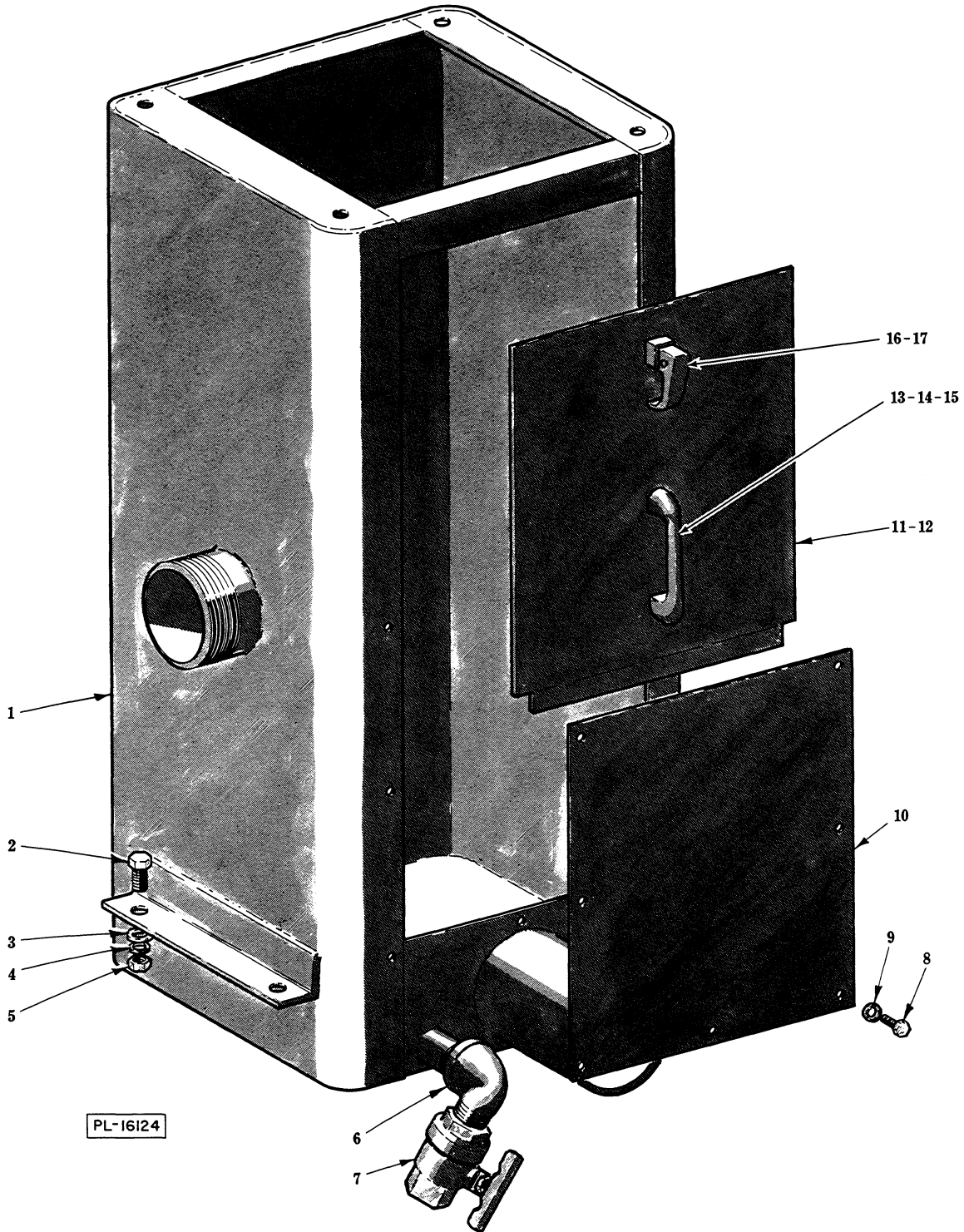
WATER PRESS HOUSING UNIT
