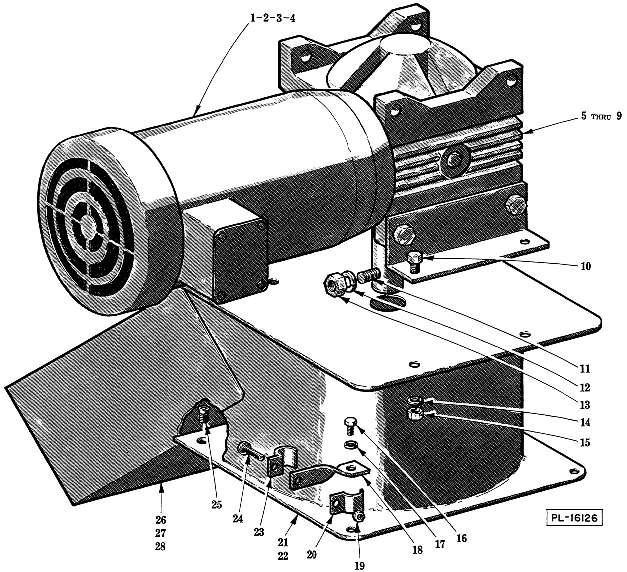
DISCHARGE UNIT
