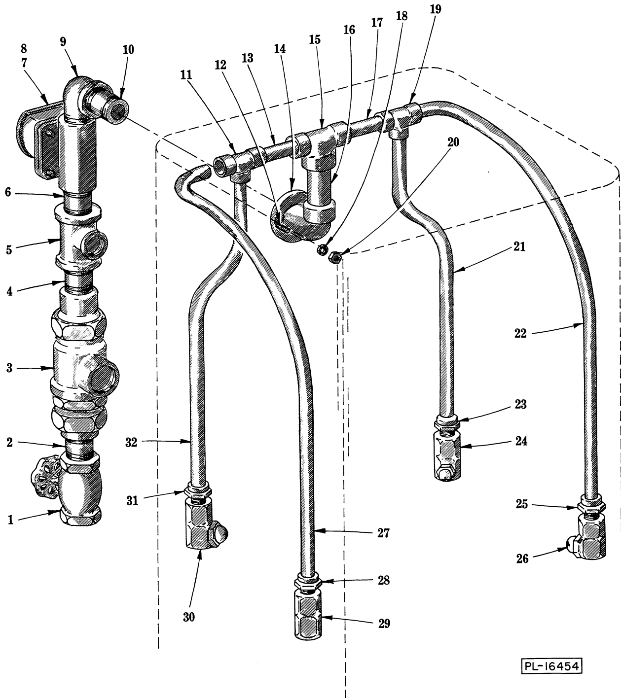
SCREEN FLUSH UNIT
