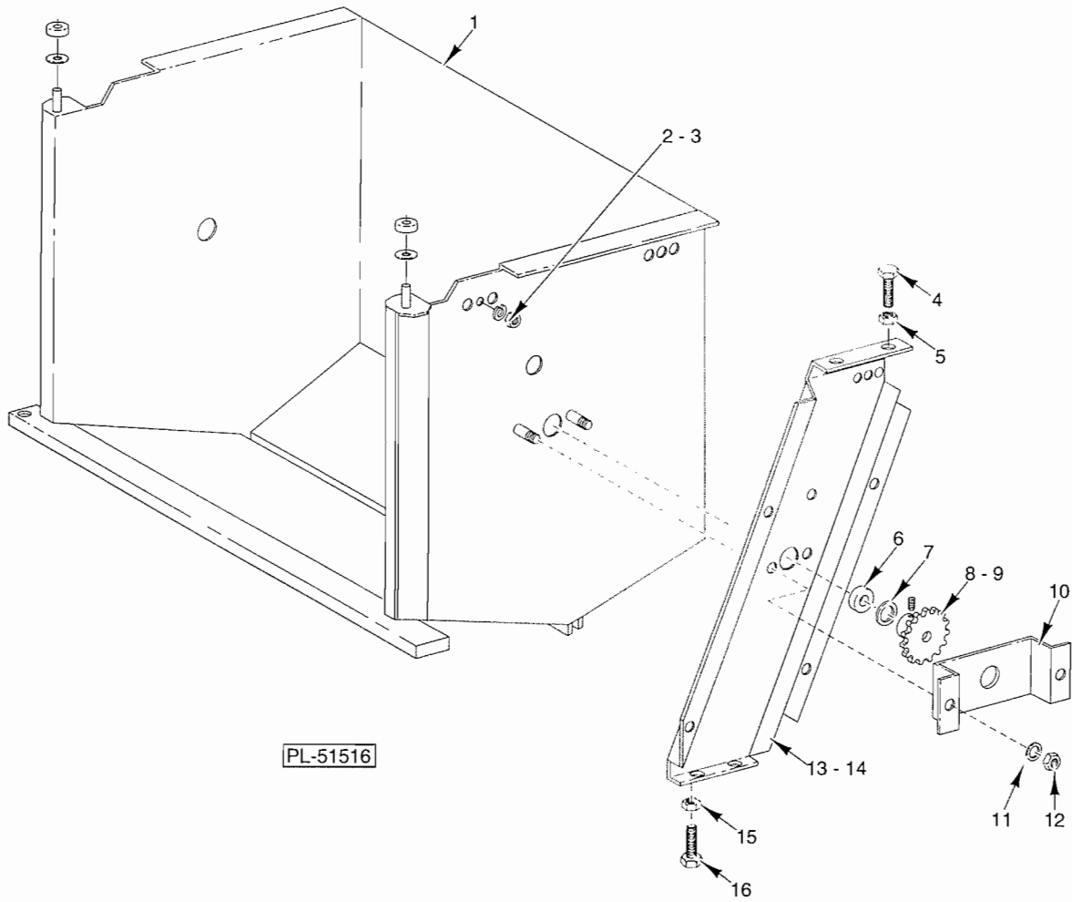
OVEN CAVITY (HRO50)
