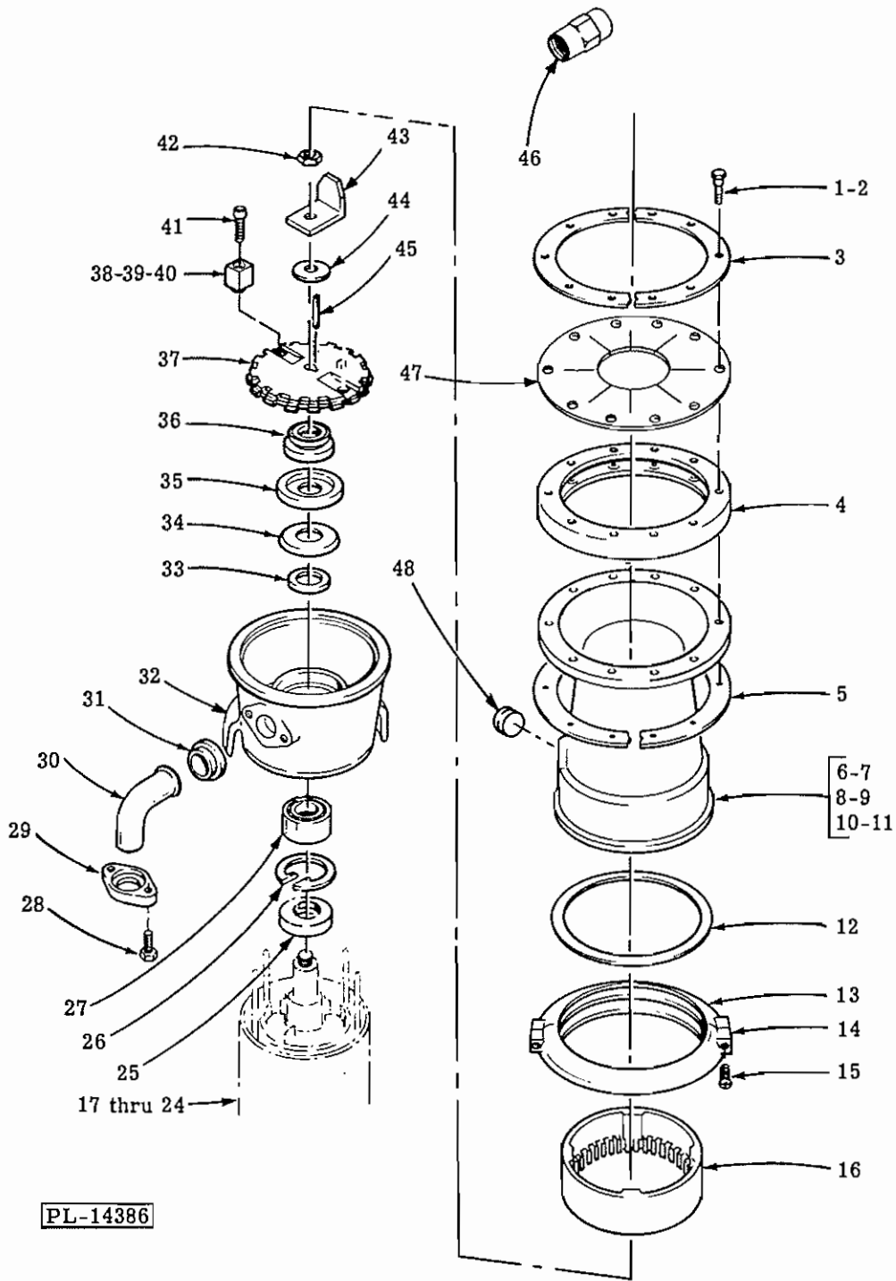
DISPOSER UNIT
