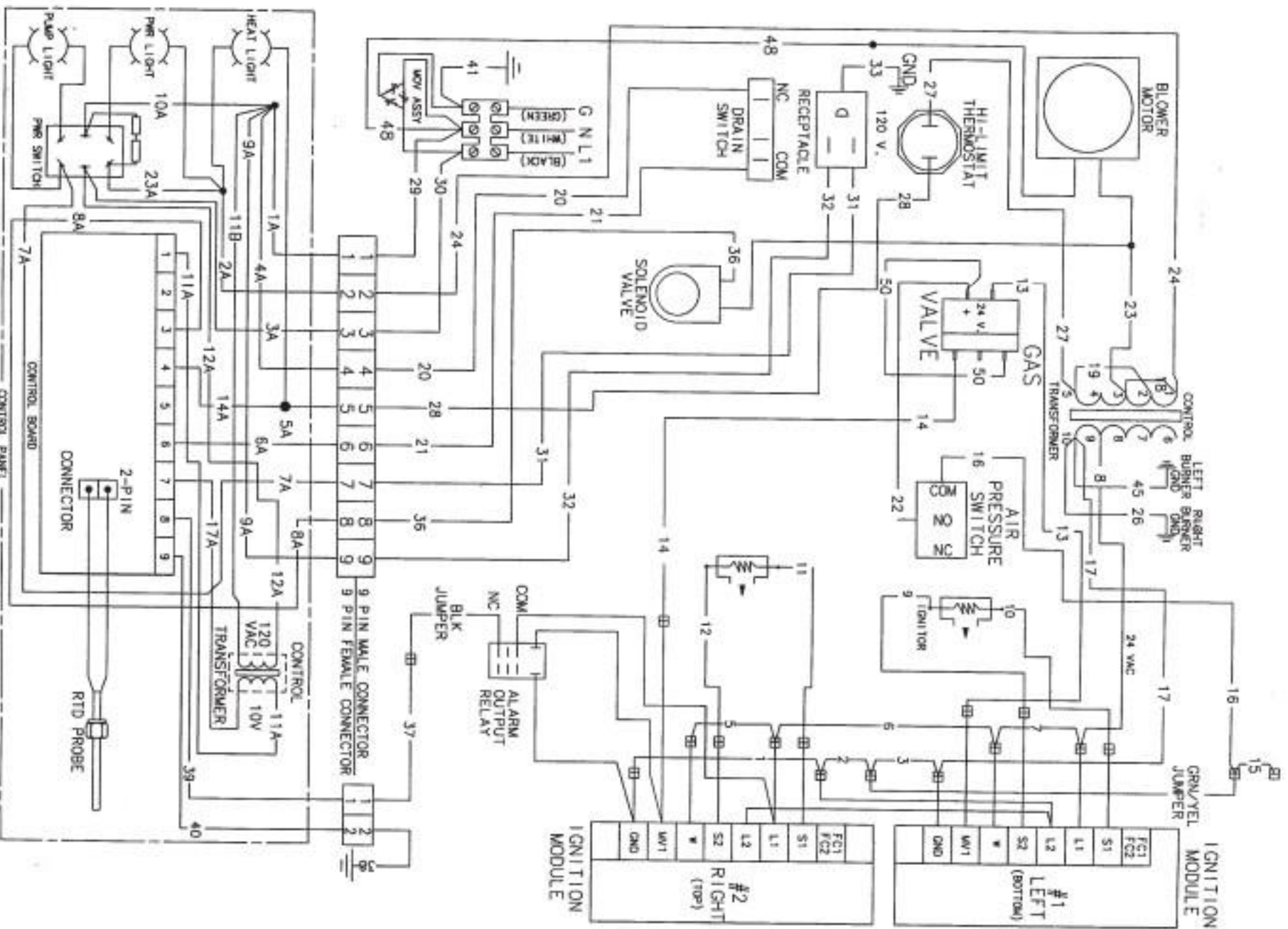
8-HEAD GAS COOKER W/LOCAL FLAME SENSING 120V 1PH 2W + G 54788
