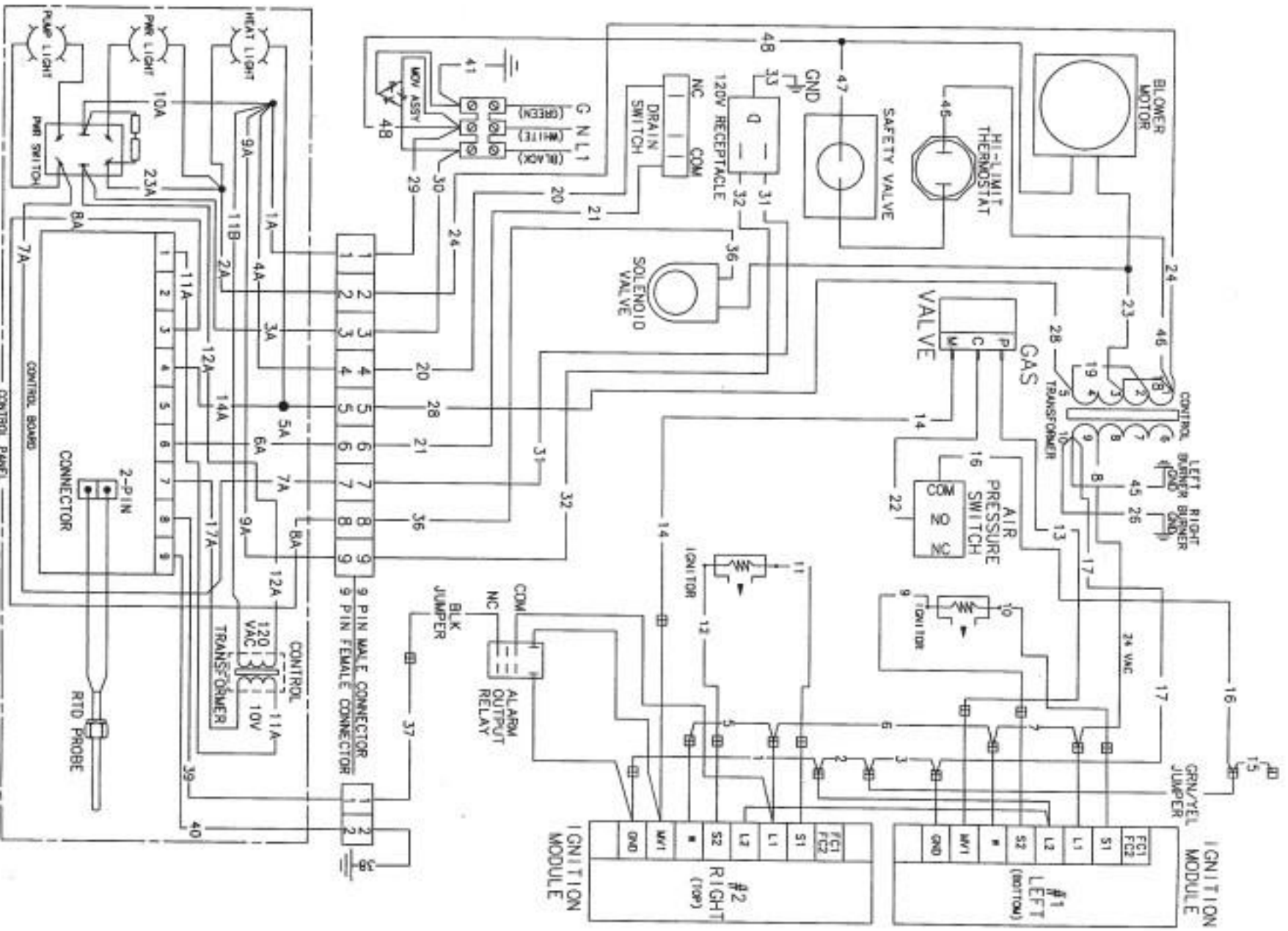
8-HEAD GAS COOKER W/LOCAL FLAME SENSING 120V 1PH 2W + G 54789
