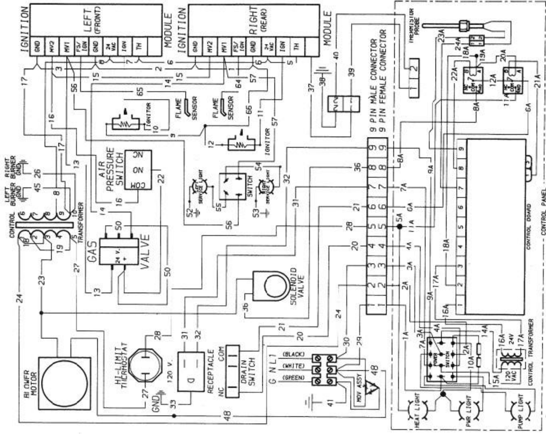
8-HEAD GAS COOKER
