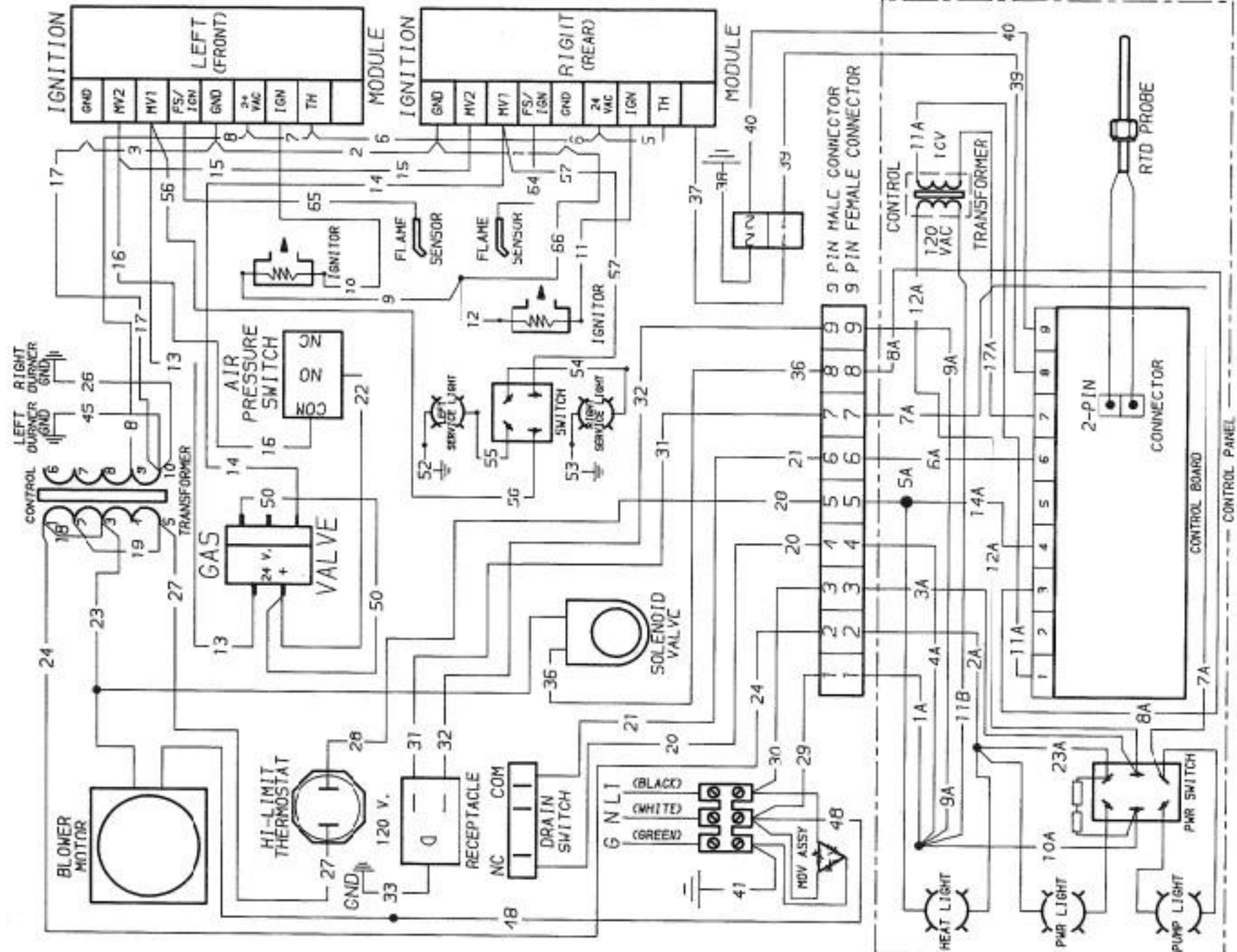
8-HEAD GAS COOKER
