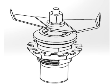
Cutter Assembly 98650
