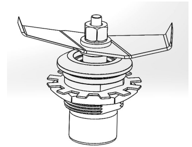
Cutter Assembly 98650
