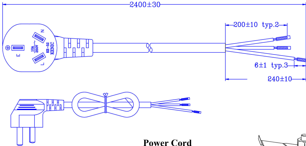
Power Cord 990167372
