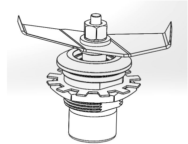
Cutter Assembly 98650
