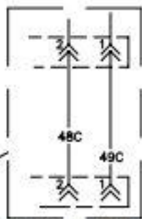
MILLIVOLT FRYER WIRING
