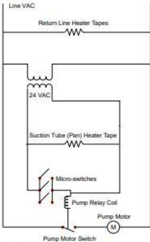
Filter Magic Simplified Wiring Diagram
