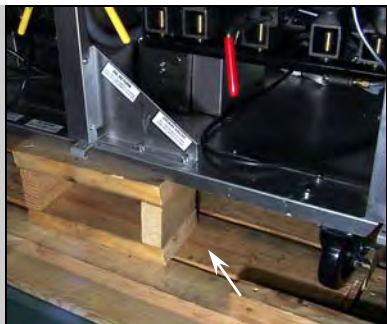
Figure 1: Remove pallet supports (arrow) before removing fryers from pallets.
