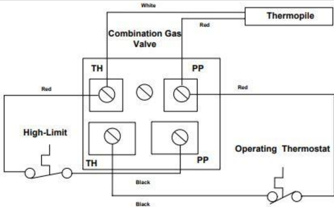
Old Style Honeywell Millivolt Gas Valve Wiring (Non-CE)
