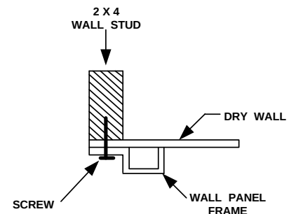
DETAIL OF WALL PANEL FRAME INSTALLATION
