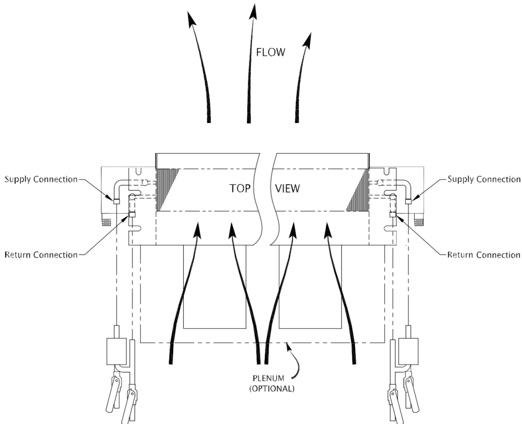
Figure 18 Determination of Right-Hand/ Left-Hand References
