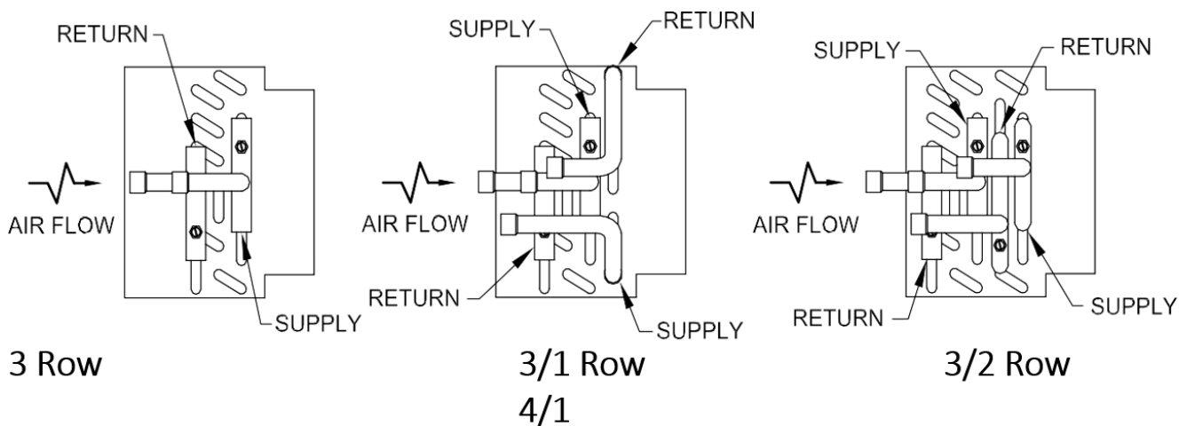
Figure 19 Coil Assemblies (Right-Hand Shown)
