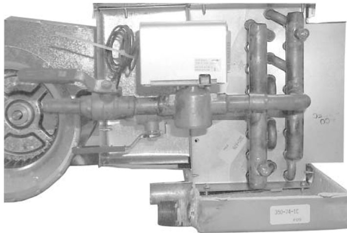
Figure 16 Two-Way Motorized Valve Assembly
