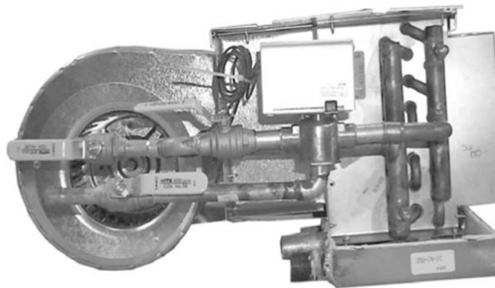
Figure 17 Three-Way Motorized Valve Assembly
