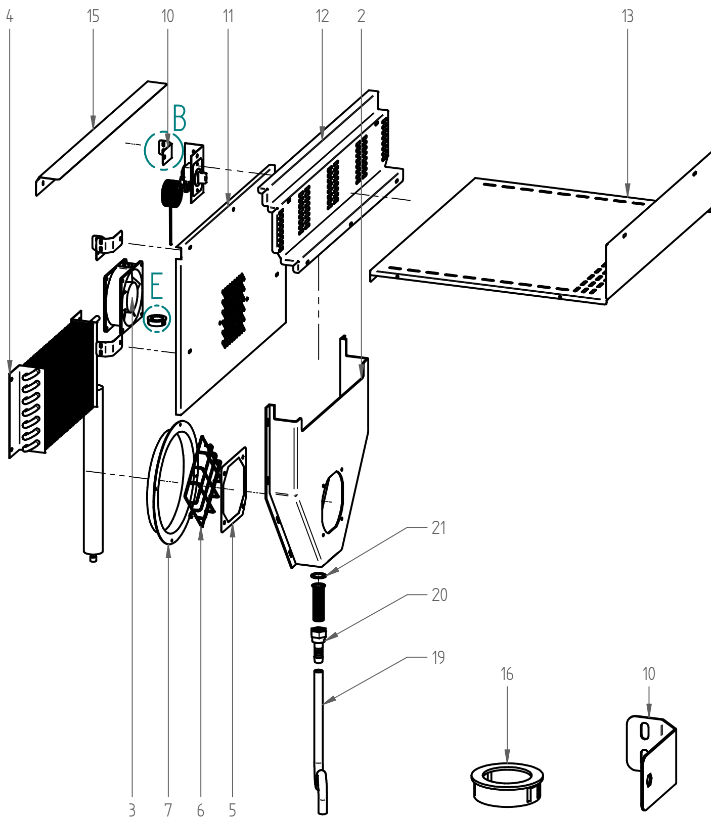
DETAIL E DETAIL B
