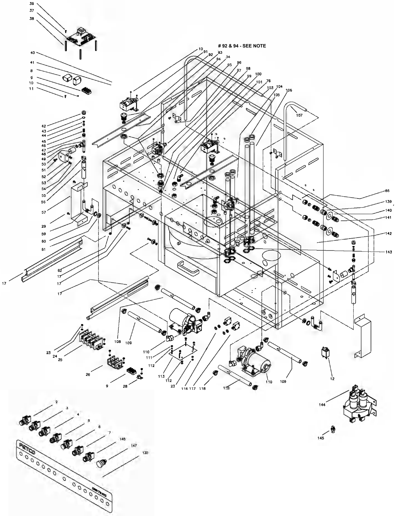
Figure 1 – CBS-72A Main Assembly
