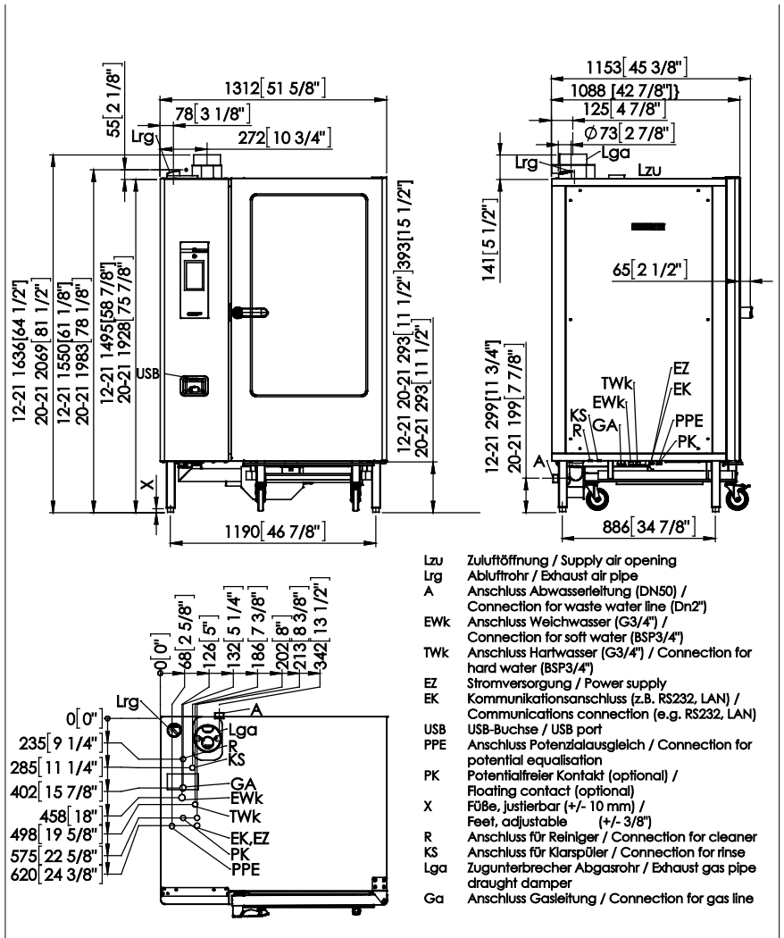
Fig. 10: Size 12-21 and 20-21, gas, right hinged
