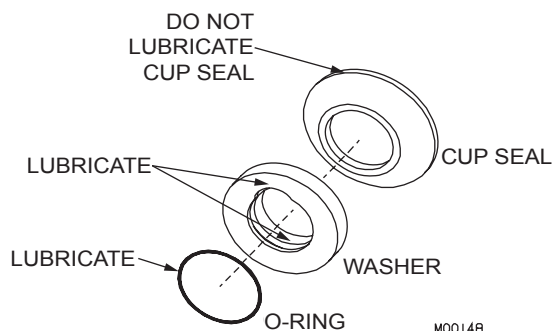
Figure 8-1 Shaft Seal Assembly
