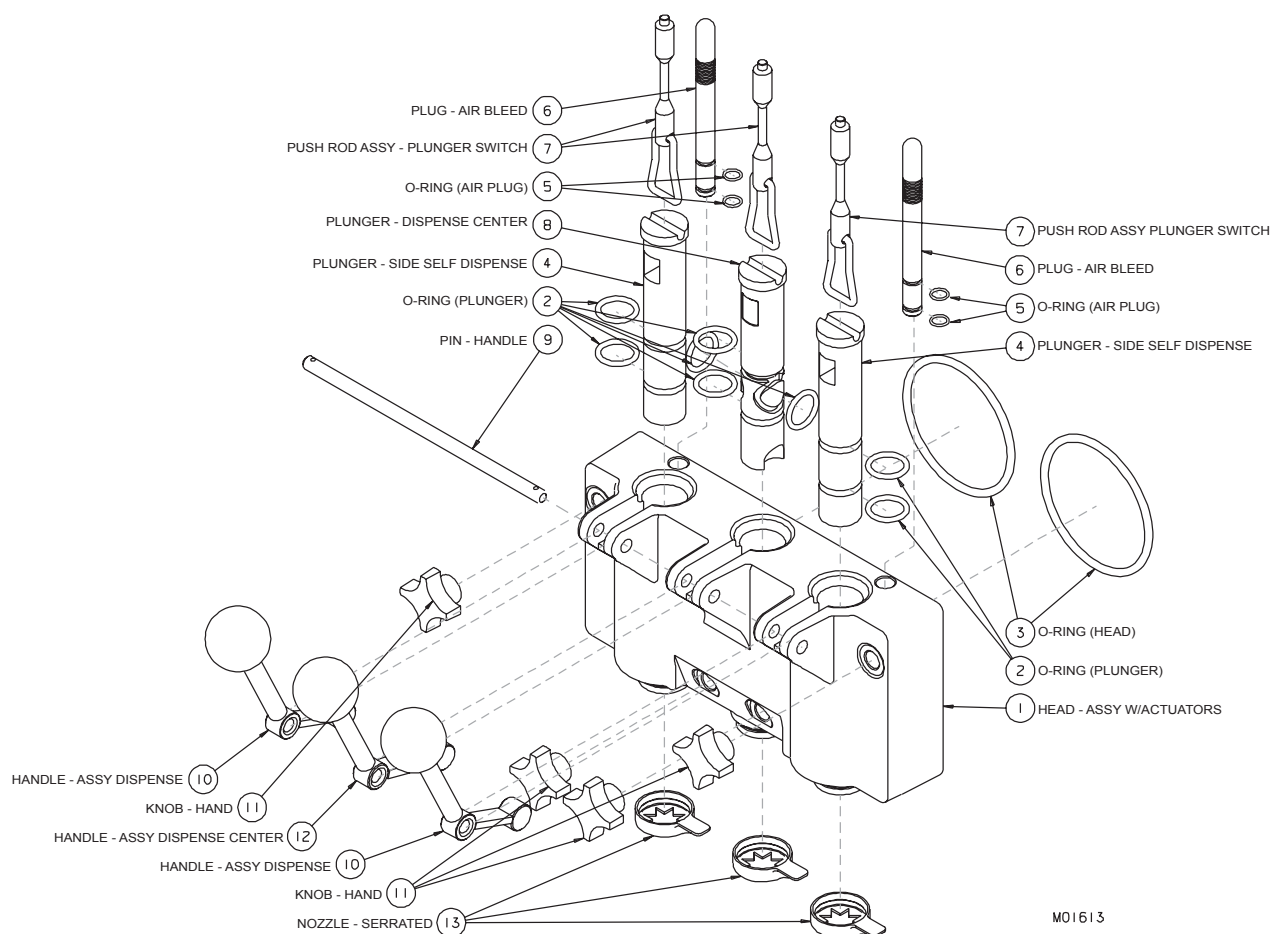
Figure 8-4 Head Assembly
