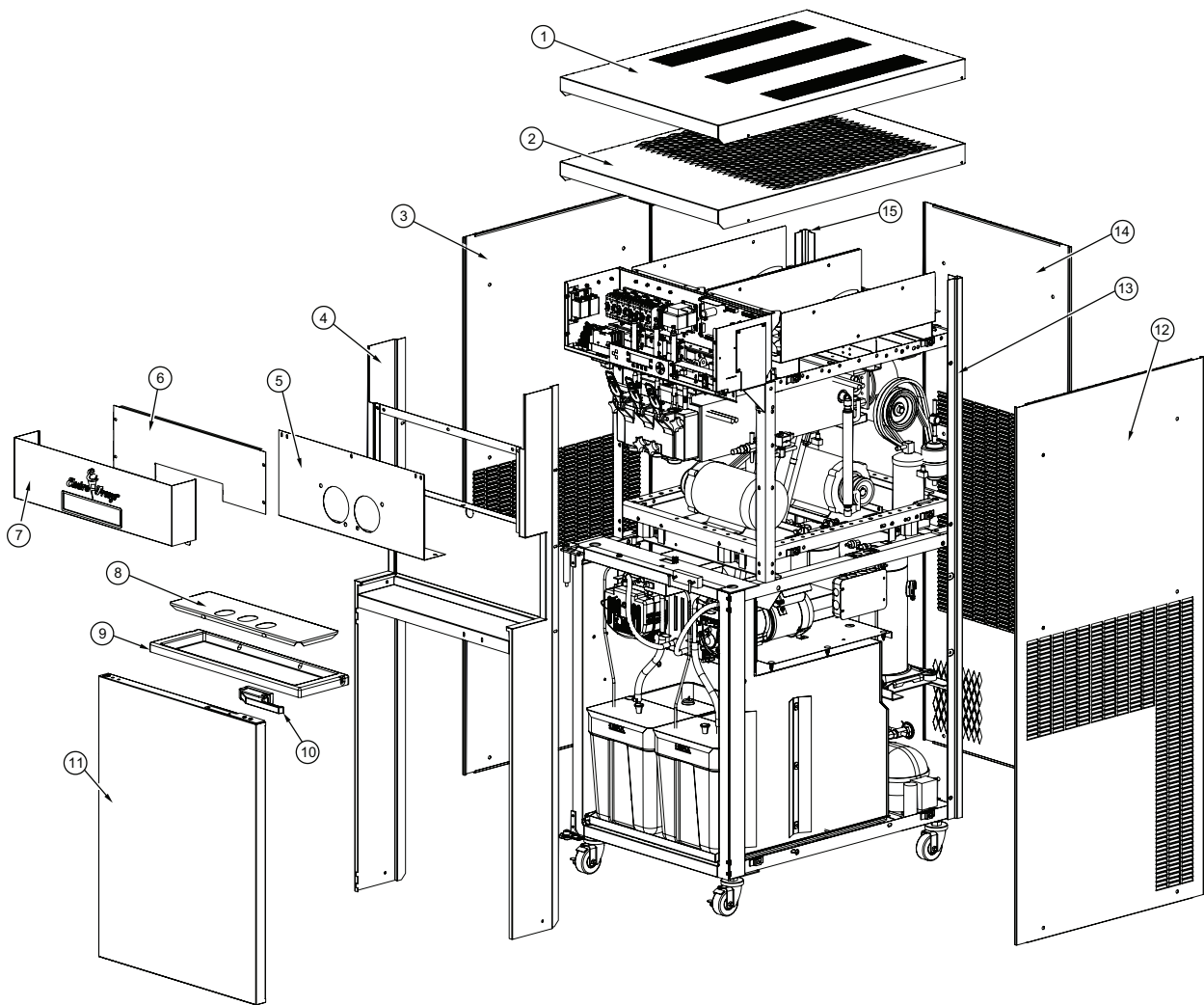
Figure 10 Panel Breakdown (Breakdown)
