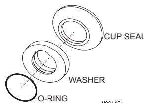
Figure 7-3 Shaft Seal
