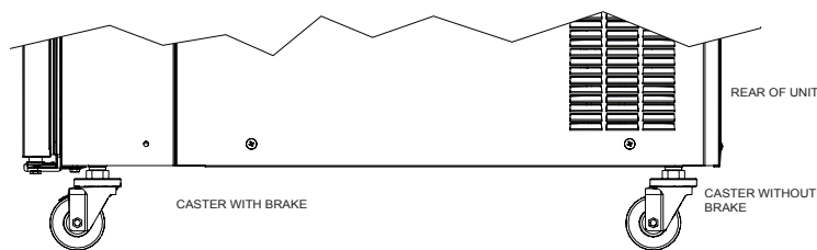
Figure 2-2 Installing Mounting Legs or Casters
