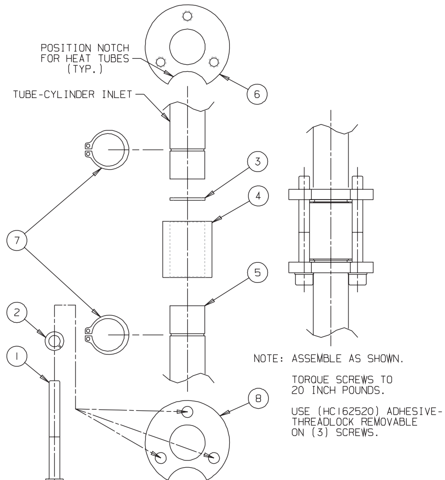
Figure 14 Mix Feed Seal Assembly
