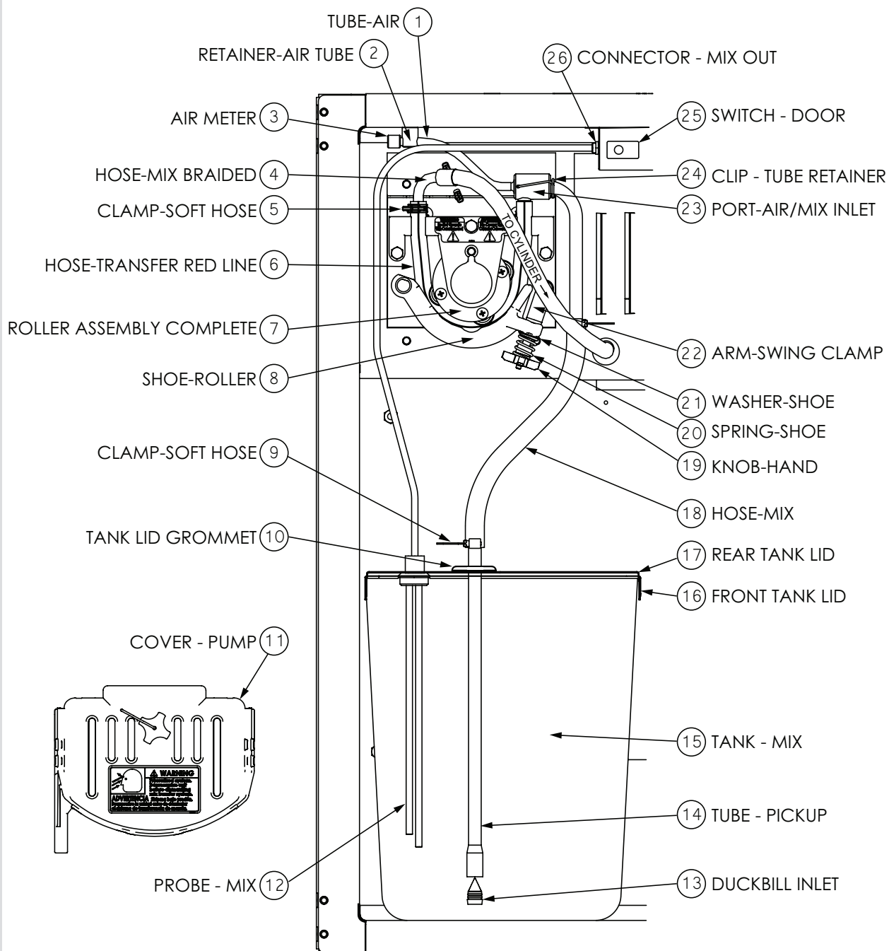
Figure 4-3 Mix Transfer System (MTS) LEFT SIDE*
