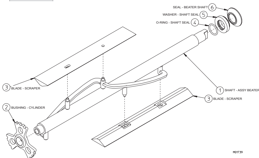
Figure 8-2 Beater Shaft Assembly
