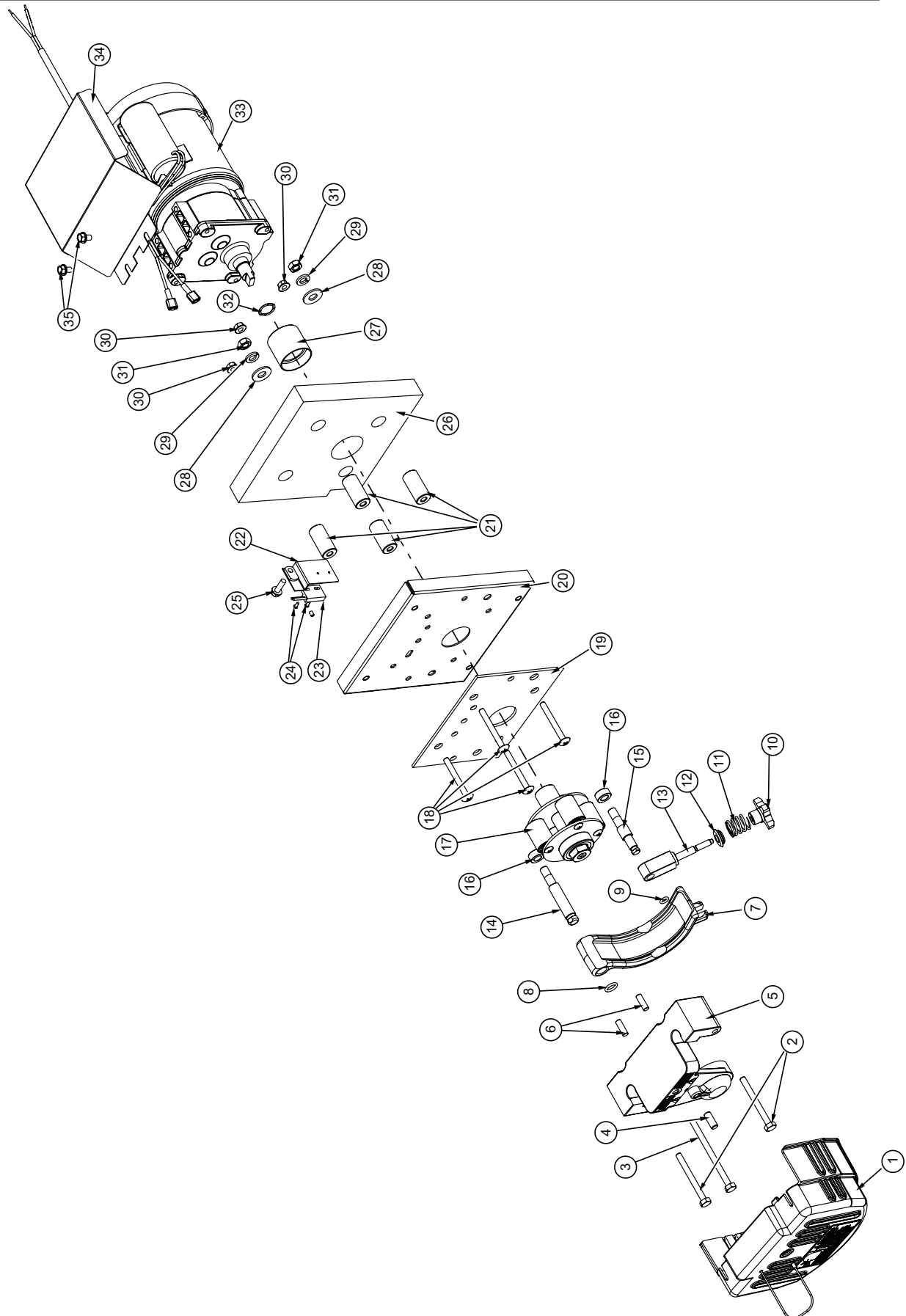
Figure 5 Mix Transfer System RMT 1Ph. (Sheet 1 of 2)
