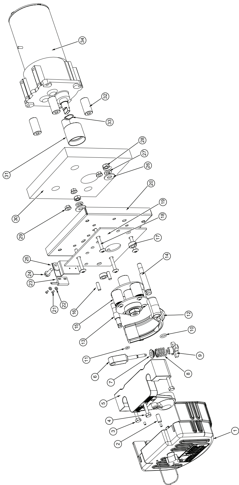
Figure 6 Mix Transfer System RMT 3Ph (sheet 1 of 2)
