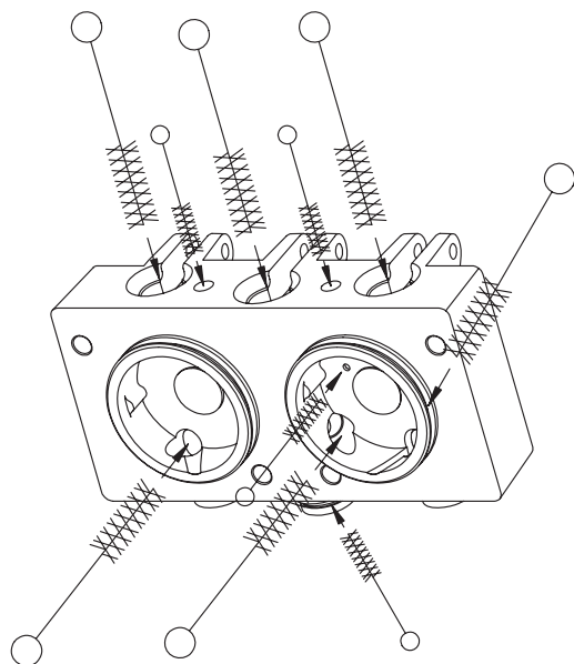
Figure 7-6 Clean head ports and openings with brush.
