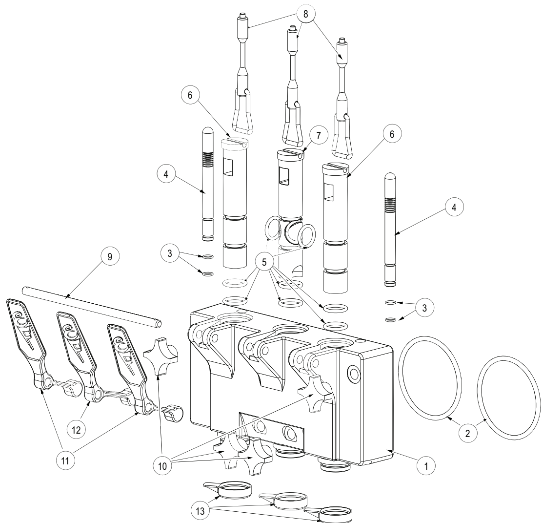
Figure 1 Head Assembly
