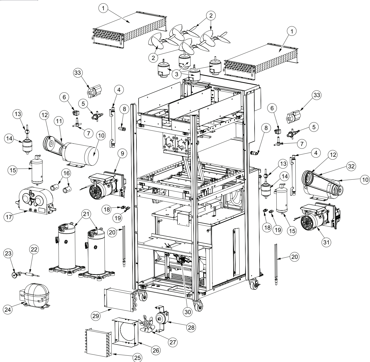
Figure 11 Air Cooled Side/Back View (Breakdown)
