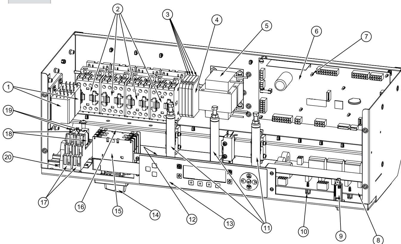
Figure 9 Switch Box (sheet 1 of 2)
