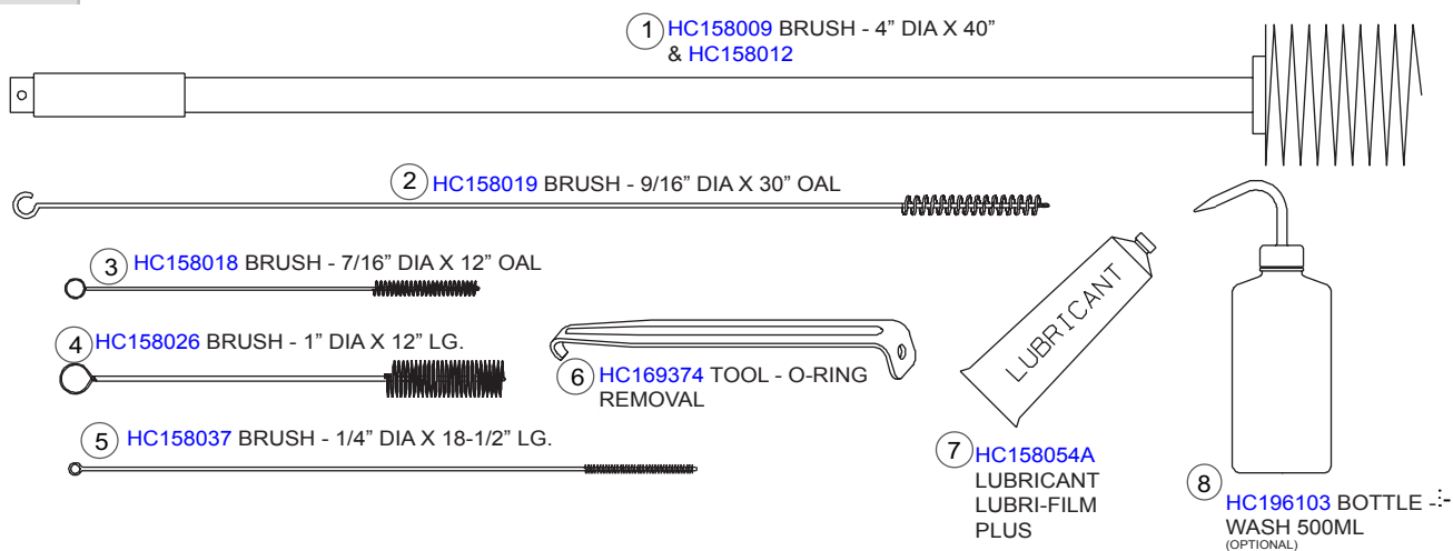
Figure 7-1 Cleaning Accessories
