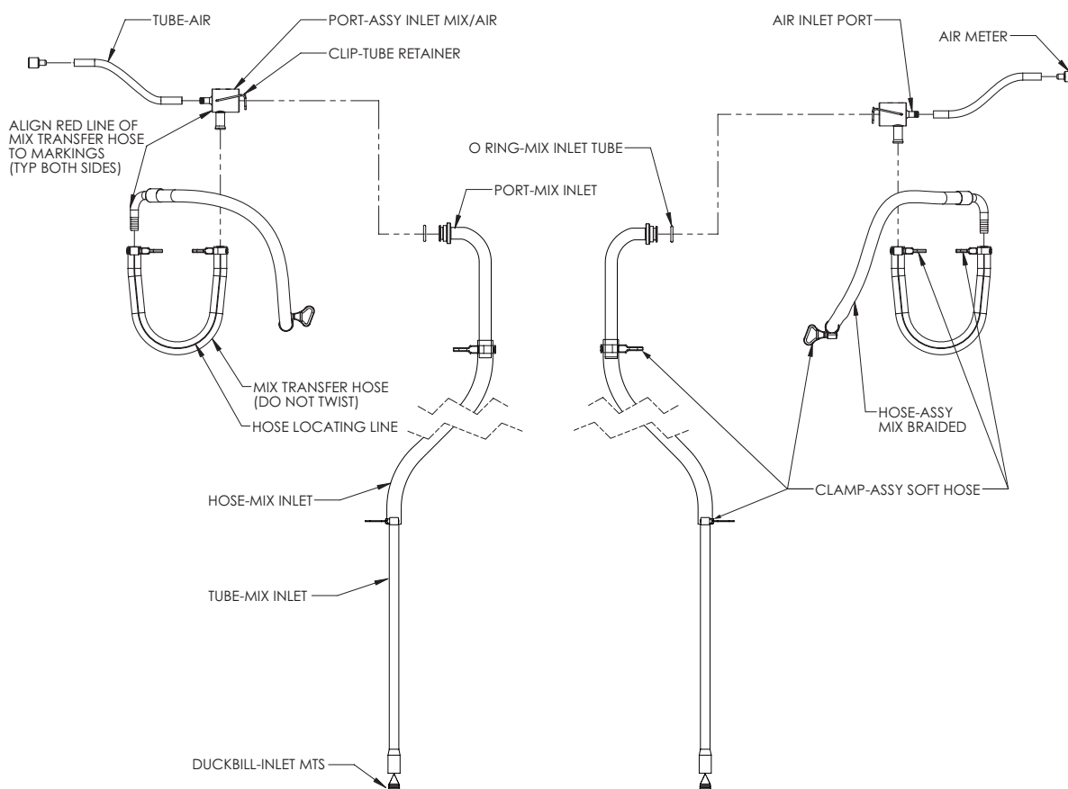
Figure 7-5 MTS Hose Assembly
