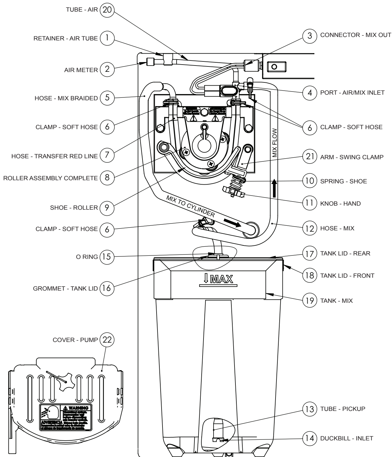
Figure 4-3 Mix Transfer System (MTS) LEFT SIDE*
