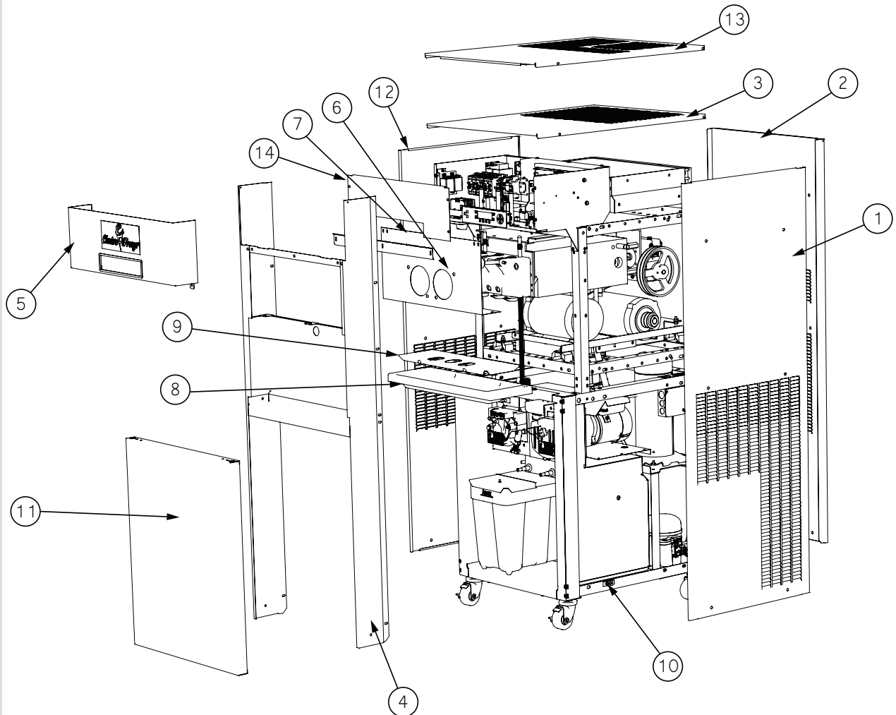
Figure 9 Panel Breakdown (Breakdown)
