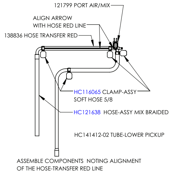
Figure 8-6 Attaching Braided Hose
