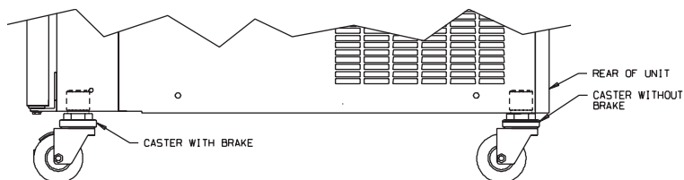
Figure 2-2 Installing Mounting Legs or Casters
