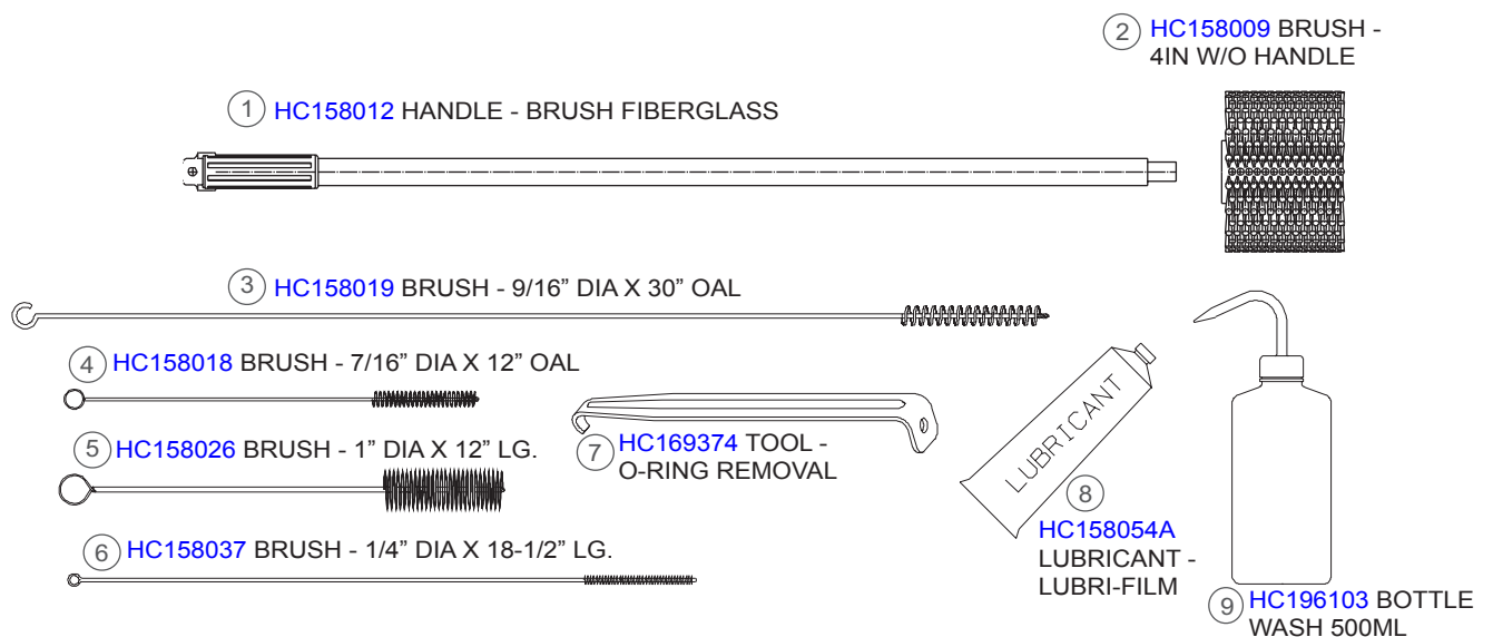
Figure 7-1 Cleaning Accessories
