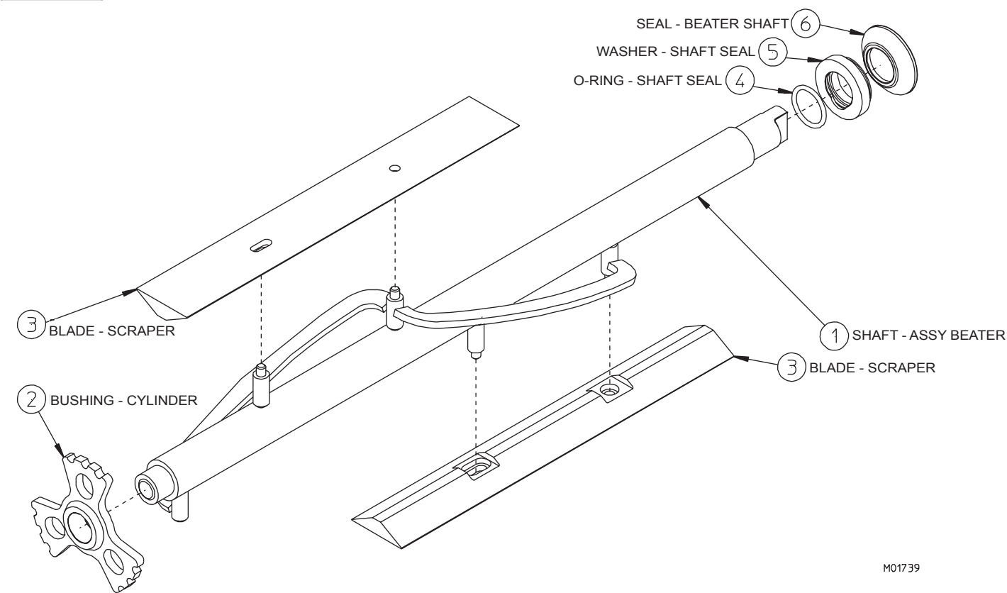
Figure 4-2 Beater Shaft Assembly
