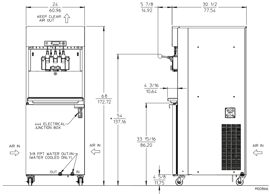
Figure 3-2 Dimensions
