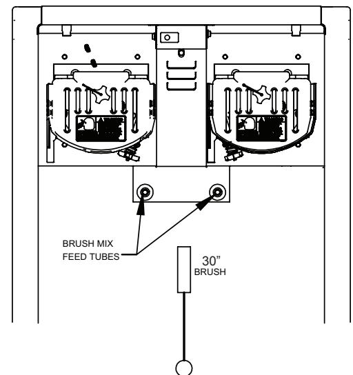
Figure 7-9 Brush inside of cylinder mix feed tubes.
