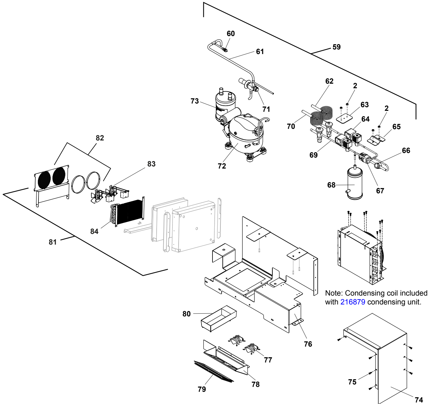
Figure: PL-2 32" Cook Station
