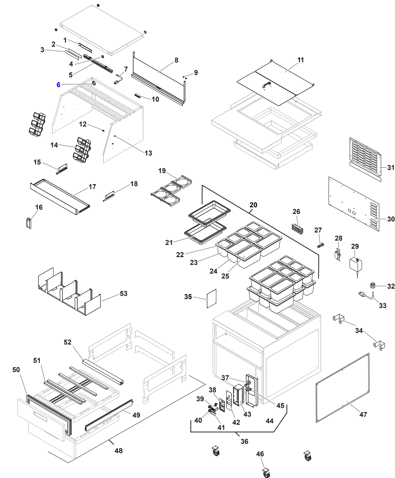
Figure: PL-9 32" Assembly Station
