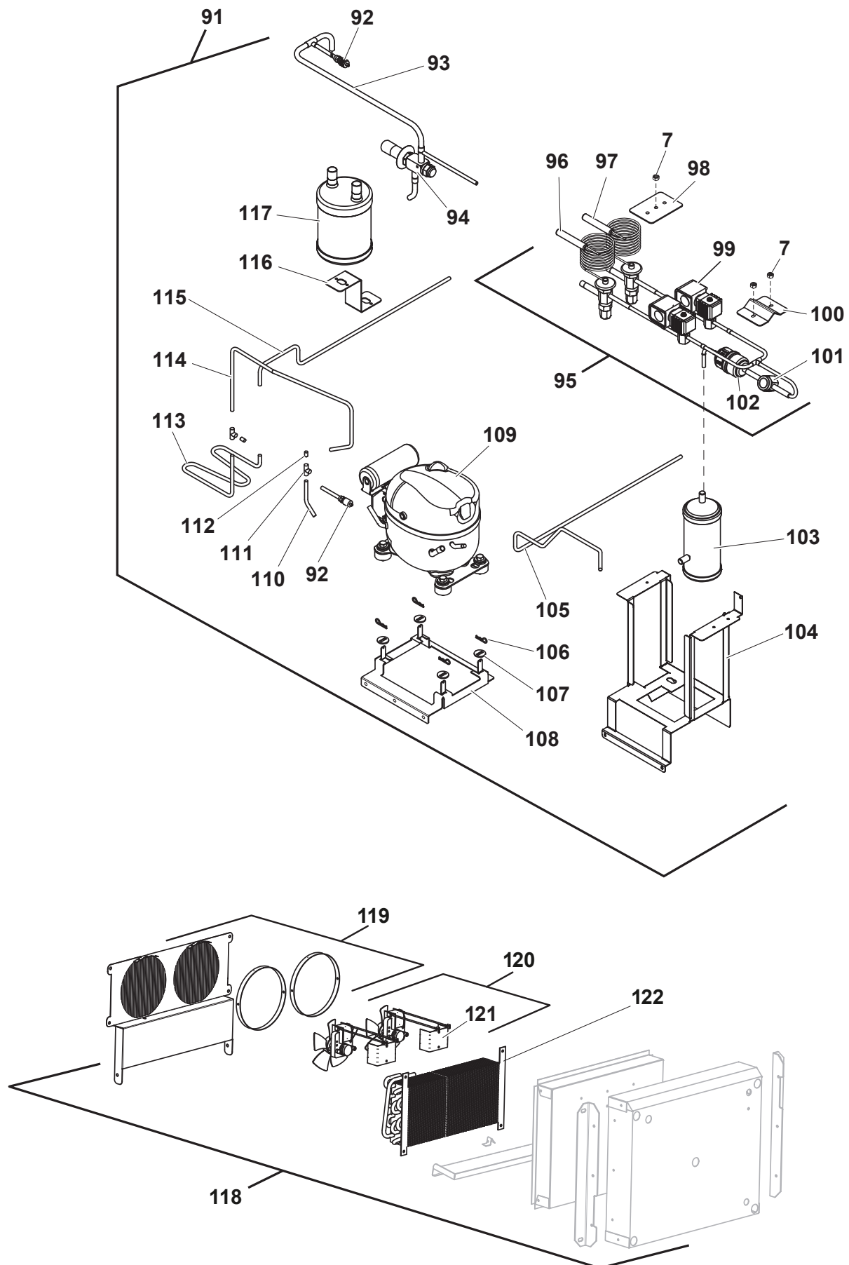
Figure: PL-13 32" Assembly Station with "KOOL" System (cont.)
