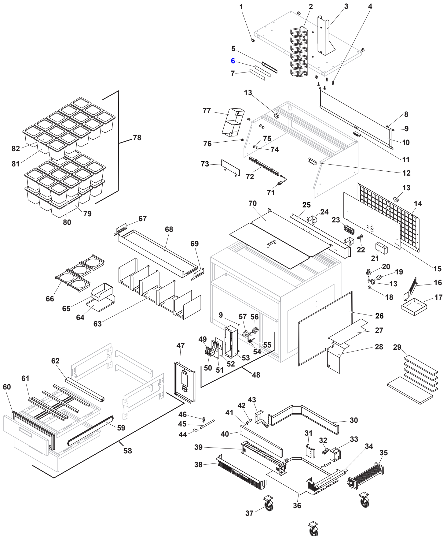
Figure: PL-7 38" Assembly Station with "KOOL" System
