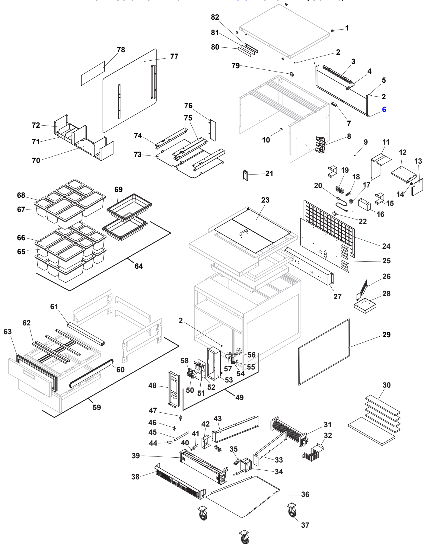
Figure: PL-3 32" Cook Station with "KOOL" System
