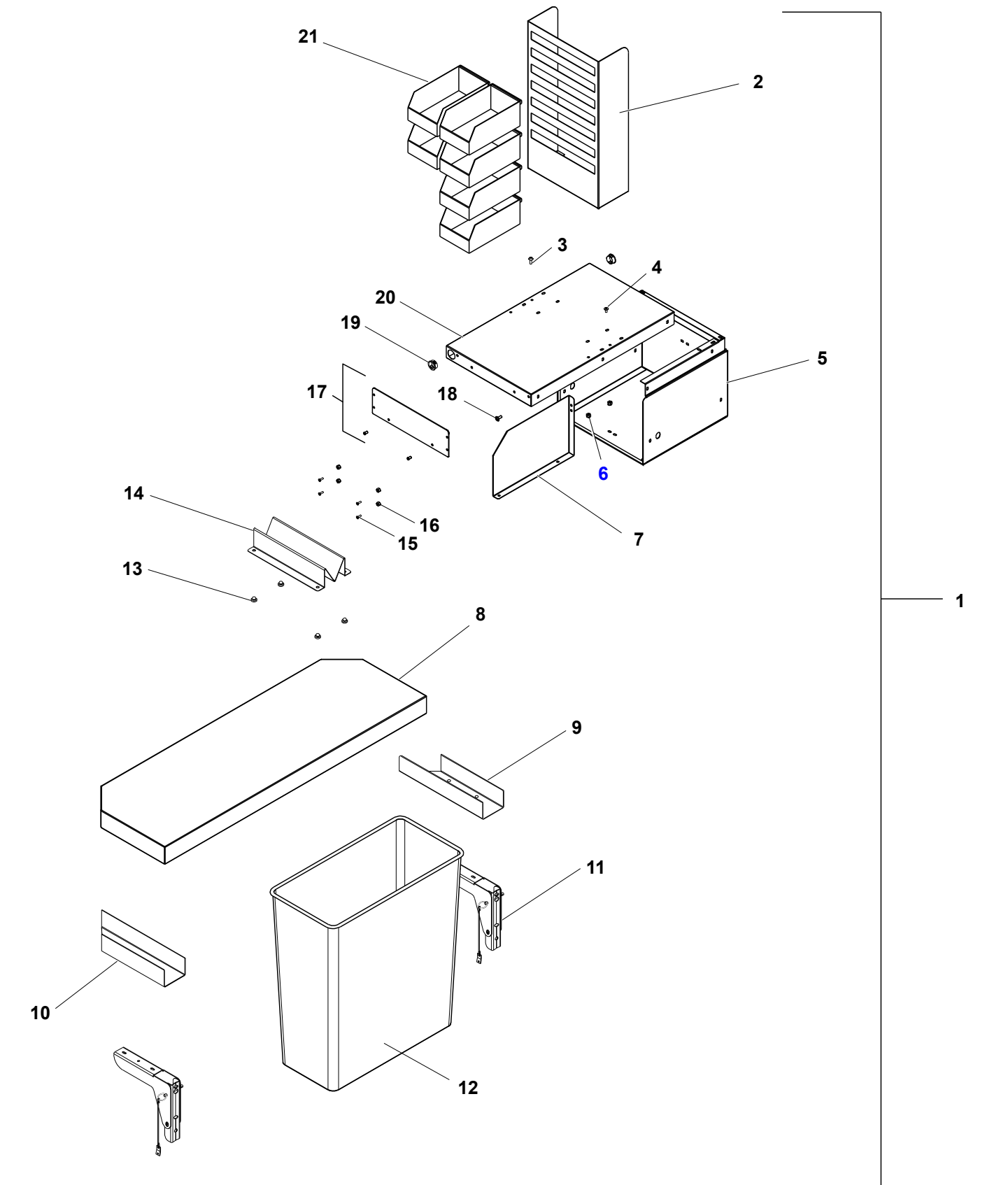
Figure: PL-11 32" Assembly Station Side Shelf Kit
