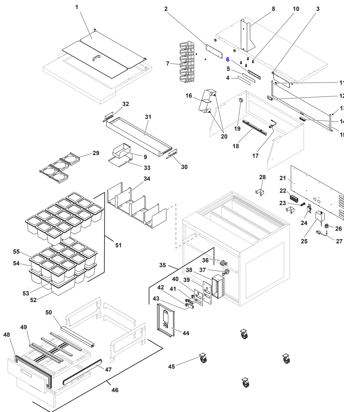
Figure: PL-5 38" Assembly Station
