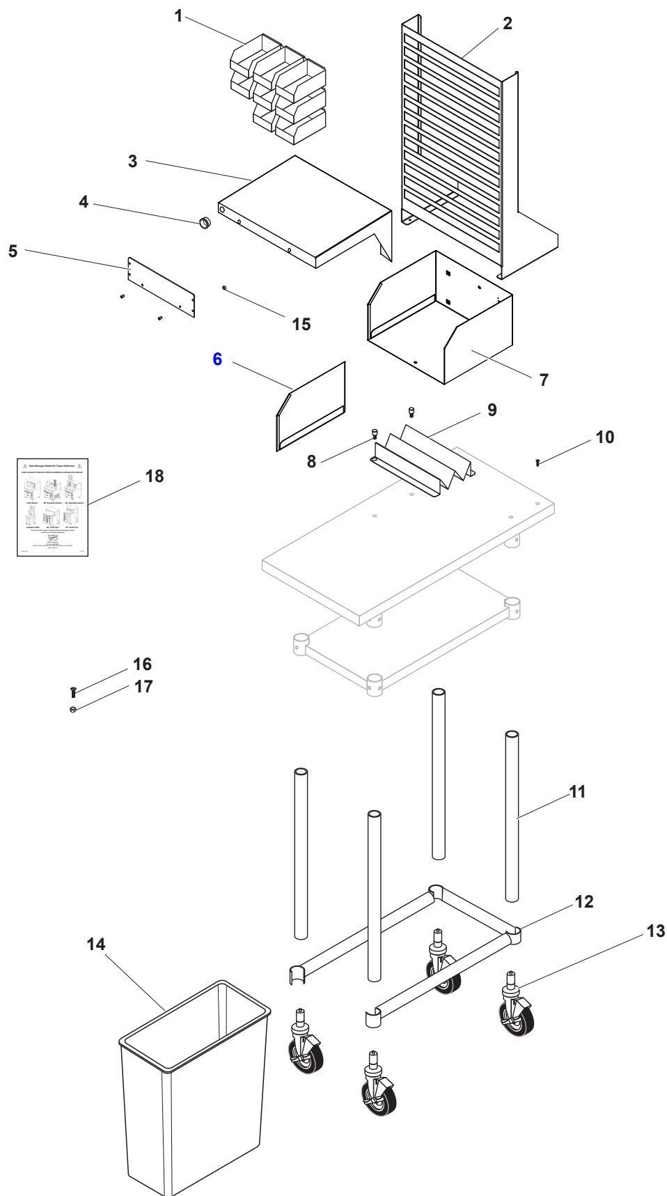
Figure: PL-16 18" Expedite Table
