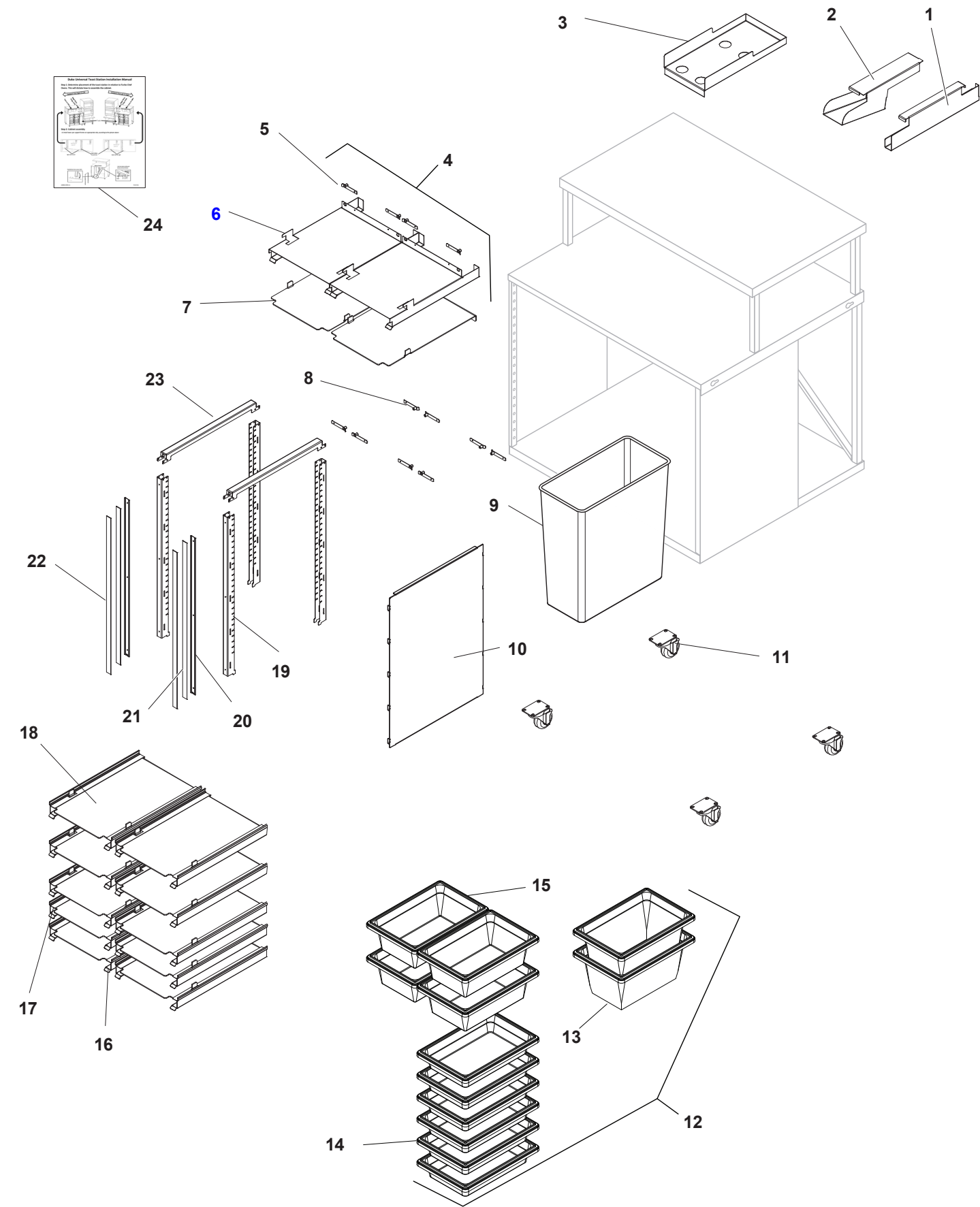
Figure: PL-14 40" Toast Station
