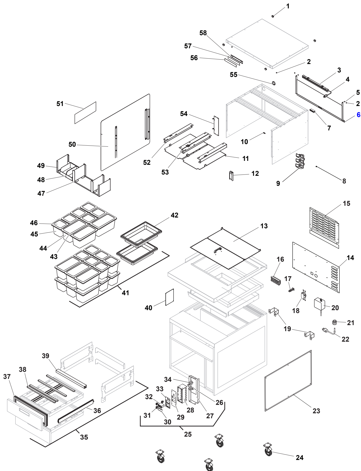
Figure: PL-1 32" Cook Station
