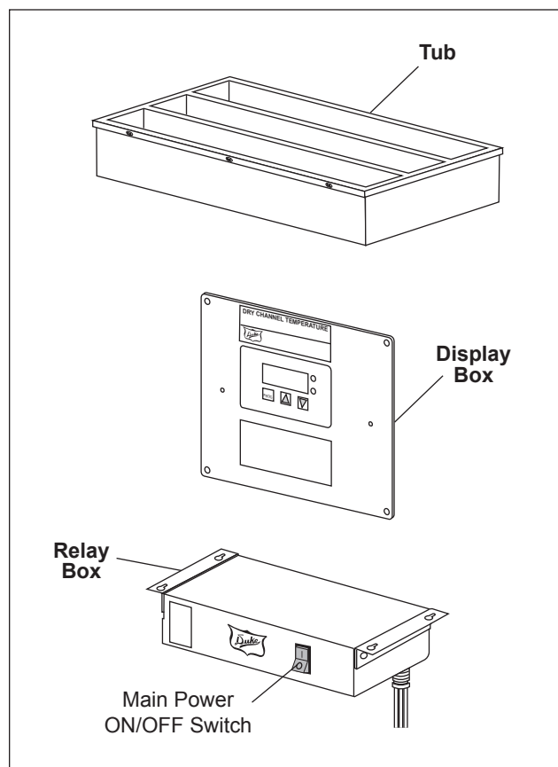
Figure 1. Dry Channel Major Components
