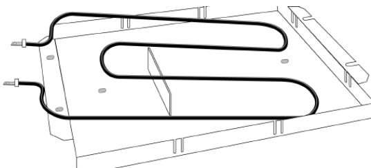
Figure 6 Element Installation
