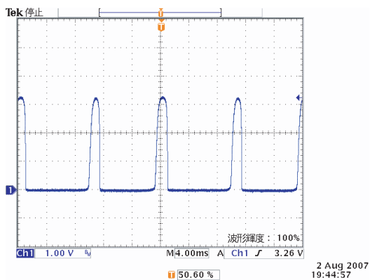
(A) Wave form1: PWR_OFF_DET 50/60 Waveform 波形1: 停電検出50/60波形 CX051 5pin (Refer to the SCHEMATIC DIAGRAMS 4/7) (SCHEMATIC DIAGRAMS 4/7を参照)
