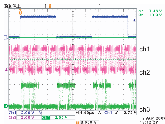
(D) Wave form 4 : A/D Waveform 波形4: A/D波形 CH1:IC300 10pin CH2:IC300 11pin CH3:IC300 32pin (Refer to the SCHEMATIC DIAGRAMS 3/7) (SCHEMATIC DIAGRAMS 3/7を参照)
