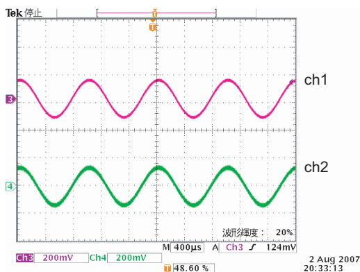
(E) Wave form 5 : Power Amp In Waveform 波形5: パワーアンプ入力波形 CH1:IC505 2pin CH2:IC505 4pin (Refer to the SCHEMATIC DIAGRAMS 6/7) (SCHEMATIC DIAGRAMS 6/7を参照)
