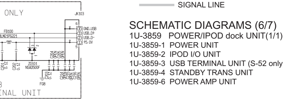
1U-3859-2 IPOD I/O UNIT
