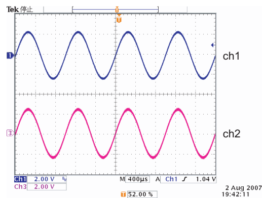
(F) Wave form 6 : Speaker In Waveform 波形6: スピーカー入力波形 CH1:CY042 1pin CH2:CY042 4pin (Refer to the SCHEMATIC DIAGRAMS 6/7) (SCHEMATIC DIAGRAMS 6/7を参照)
