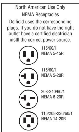
Figure 3. Receptacle Configurations
