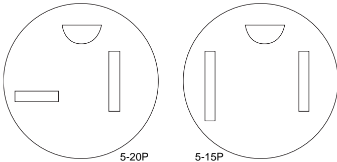
5-20P and 5-15P Electrical Plug Configurations
