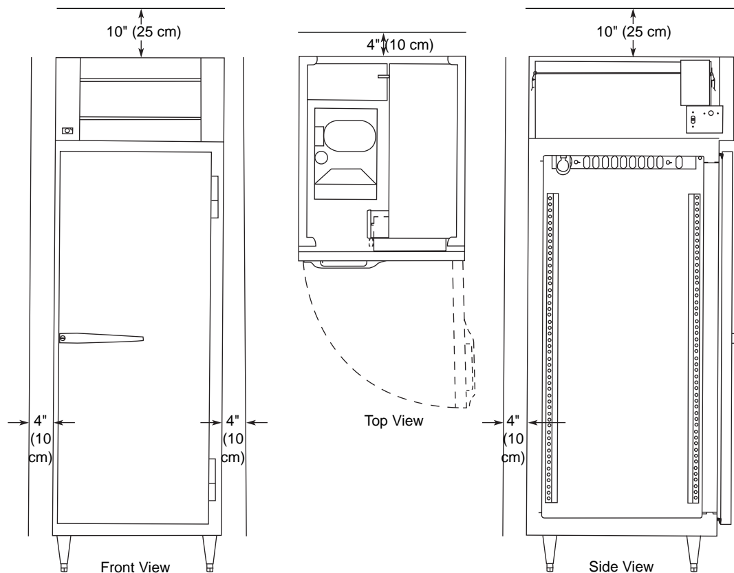
Cabinet Clearances (Typical Single Door Cabinet Shown)
