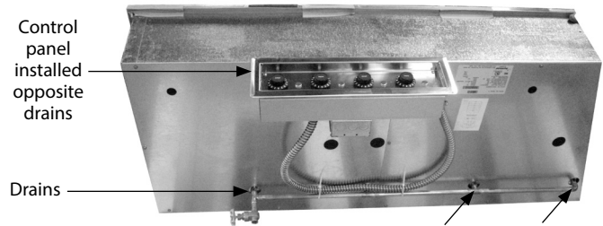
Infinite control shown, directions also apply to digital control
