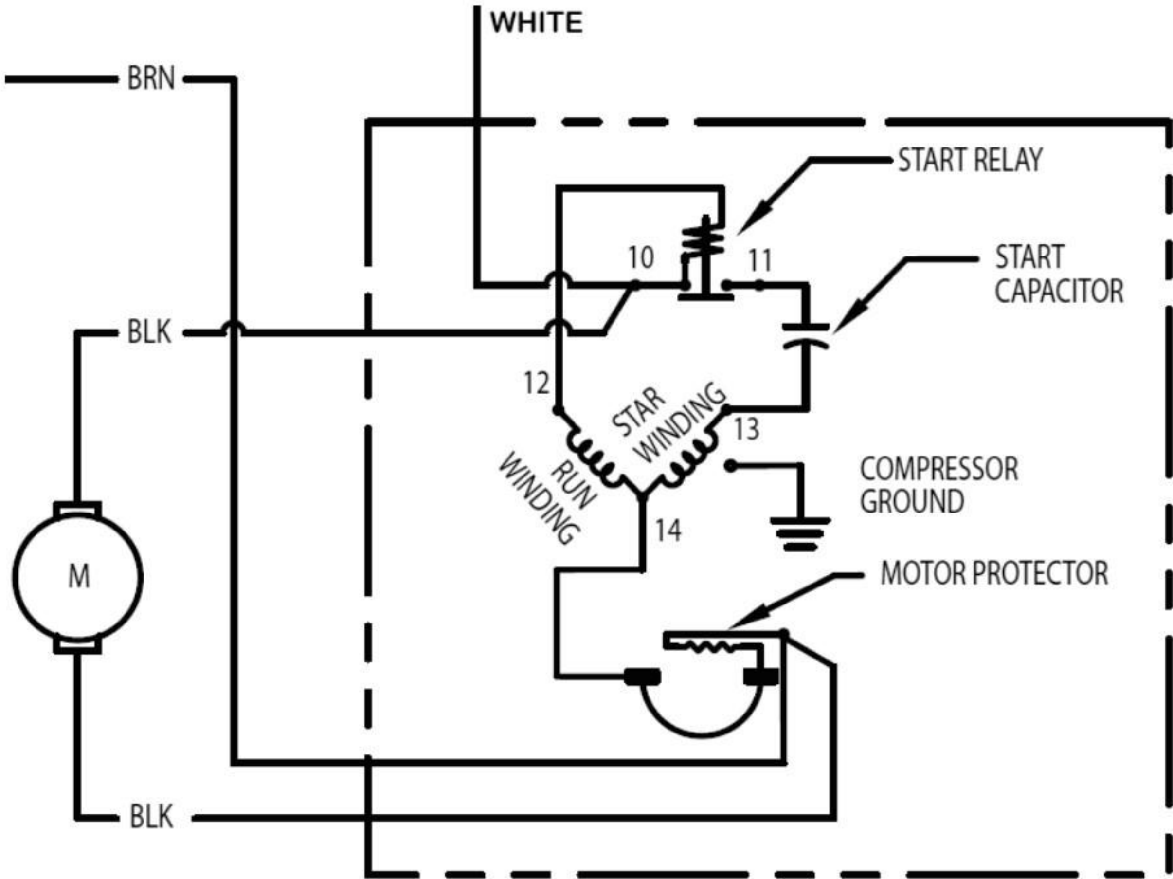
COMPRESSOR
